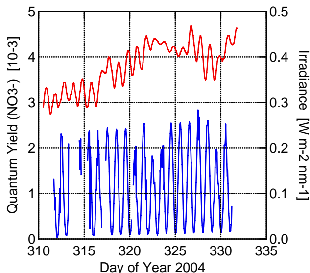
Fig. 6. The measured downwelling surface irradiance recorded throughout the campaign at 350 nm (blue, units of \text{W m}^{-2} \text{ nm}^{-1} , right scale). Also plotted is the calculated quantum yield for nitrate photolysis to yield \text{NO}_2 in ice (Reaction 1, units of 10^{-3} , red, left scale). The variation of the quantum yields is due to the temperature of the snowpack recorded at 12.5 cm depth throughout the campaign.
