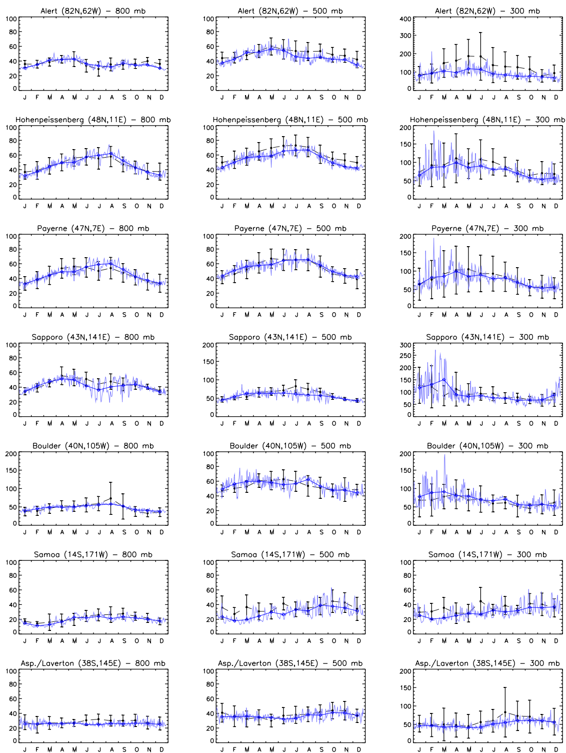
Fig. 15. Measured (solid circles) and calculated (solid light blue lines indicate day-to-day variations, open diamonds denote monthly mean values) seasonal cycle of \text{O}_3 mixing ratios (ppbv) at 7 stations and at the 800, 500, and 300 hPa levels. Observations were compiled by Logan (1999).
