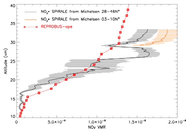
Fig. 4. Vertical profiles of reconstructed NO y * compared to the Reprabus model output on 2 October 2002 (red line). Black curve: NO y * profile inferred from the N 2 O-NO y correlation determined by Michelsen et al. (1998) in the 28–46° N latitude band. Orange curve: NO y * profile inferred from the correlation valid in the 3–10° N latitude band (only represented above 29 km where the air seems to mostly originate from low latitudes).
