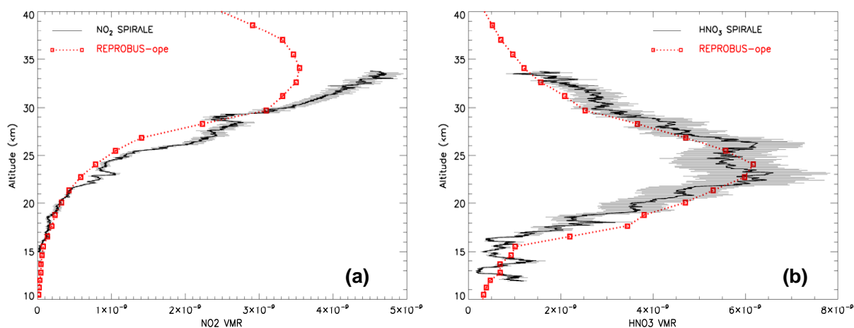
Fig. 3. Comparison between measured vertical profiles of NO 2 (a) and HNO 3 (b) on 2 October 2002 at mid-latitudes (black lines) and profiles simulated by the Reprabus 3-D CTM between 07:30 UT and 08:30 UT with a solar zenith angle varying from 64° to 74° (red lines). The model is computed using ECMWF operational analysis data.
