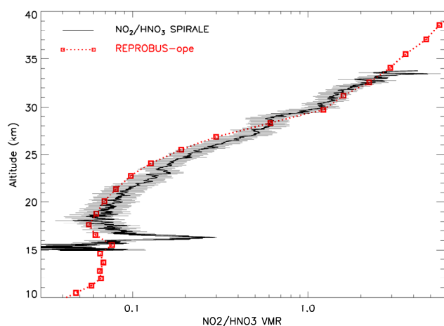
Fig. 5. NO 2 /HNO 3 ratio measured by SPIRALE (black line) and calculated by Reprobis 3-D CTM between 07:30 UT and 08:30 UT (red line). The model is driven by ECMWF 6-hourly operational analysis.
