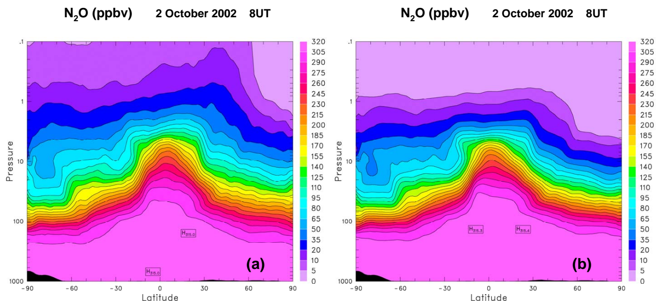
Fig. 6. N 2 O zonal means simulated by Reprobis on 2 October 2002 at 08:00 UT. (a) Results obtained using 6-hourly ECMWF operational analysis data; (b) Results obtained using 3-hourly analysed and forecast data (see text).
