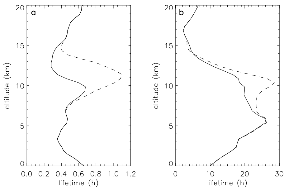
Fig. 11. Same as Fig. 9 but for isoprene.
