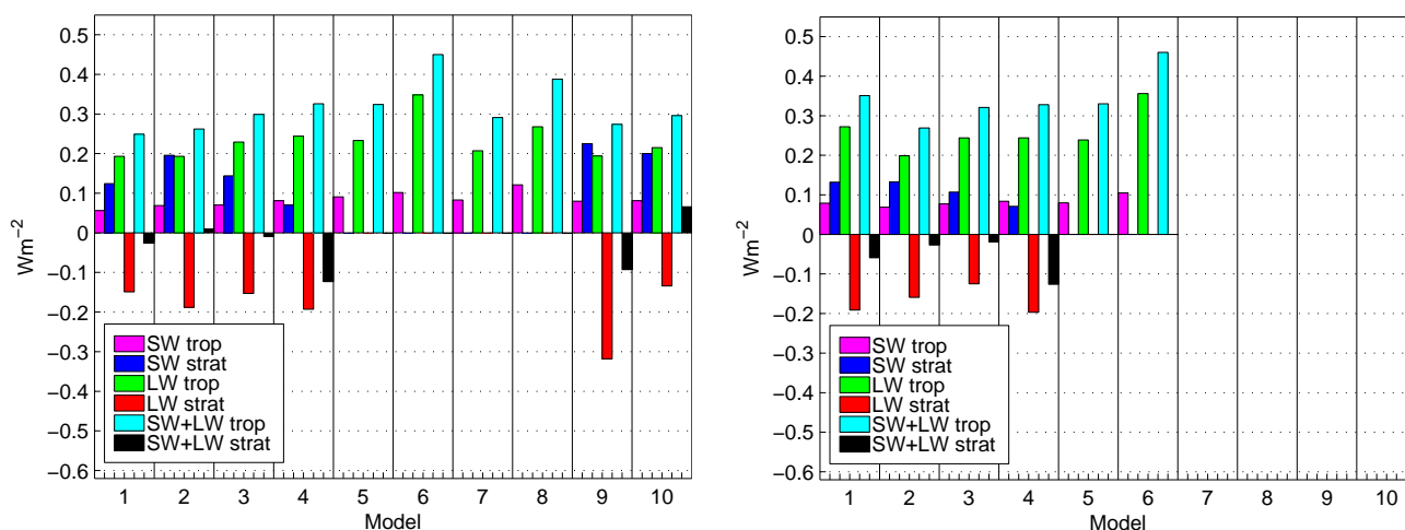
Fig. 8. Components of global-mean adjusted radiative forcing ( \text{Wm}^{-2} ) between 1850 and 2000. “SW”: shortwave component, “LW”: longwave component, “trop”: due to tropospheric ozone change, “strat” due to stratospheric change. (a) “2 minus 1c” (for LMDzINCA, UM_CAM, and STOCHEM.HadAM3 “2 minus 1b” is shown), (b) “2 minus 1” (for UM_CAM “2 minus 1d” is shown). Radiative forcing due to stratospheric change is shown only for the models that calculate stratospheric chemistry explicitly. Model numbering as in Table 1. For “2 minus 1” only coupled CCMs are shown. The radiative forcing calculations are made by the UiO-RTM, and the tropopause level is based on the NCEP year 2000 reanalysis.
