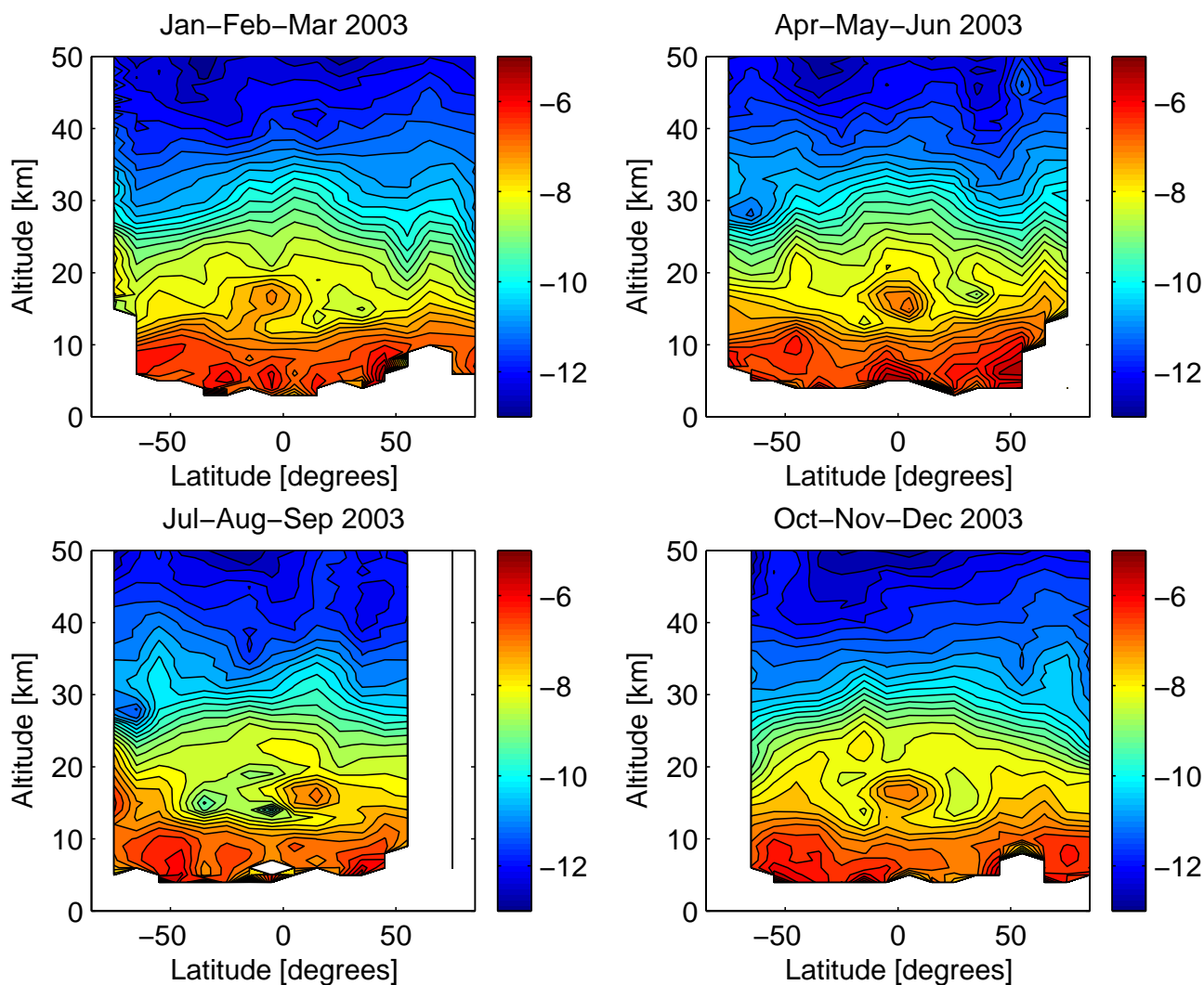
Fig. 1. The natural logarithm of the 500 nm aerosol extinction median values for 4 different periods of the year 2003. From top left to bottom right: January/February/March, April/May/June, July/August/September, October/November/December 2003. Notice the movement of the maximum in the tropics, and the appearance of Polar Stratospheric Clouds in the Antarctic lower stratosphere during July/August/September.
