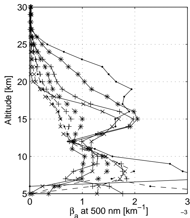
Fig. 3. The 500 nm aerosol extinction median values for June (dots), July (asterisks), August (+) and September (x) 2003, inside ( 75^{\circ} S; solid lines) and outside ( 65^{\circ} S; dashed lines) the South polar vortex. Data for the 85^{\circ} S bin were not available for these months. The PSC signature is clearly present in the lower stratosphere above 12 km.
