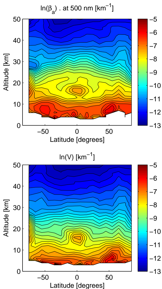
Fig. 2. Top: the natural logarithm of the 500 nm aerosol extinction median values for the year 2003. Bottom: the 500 nm aerosol extinction variability as defined in Eq. (2).
