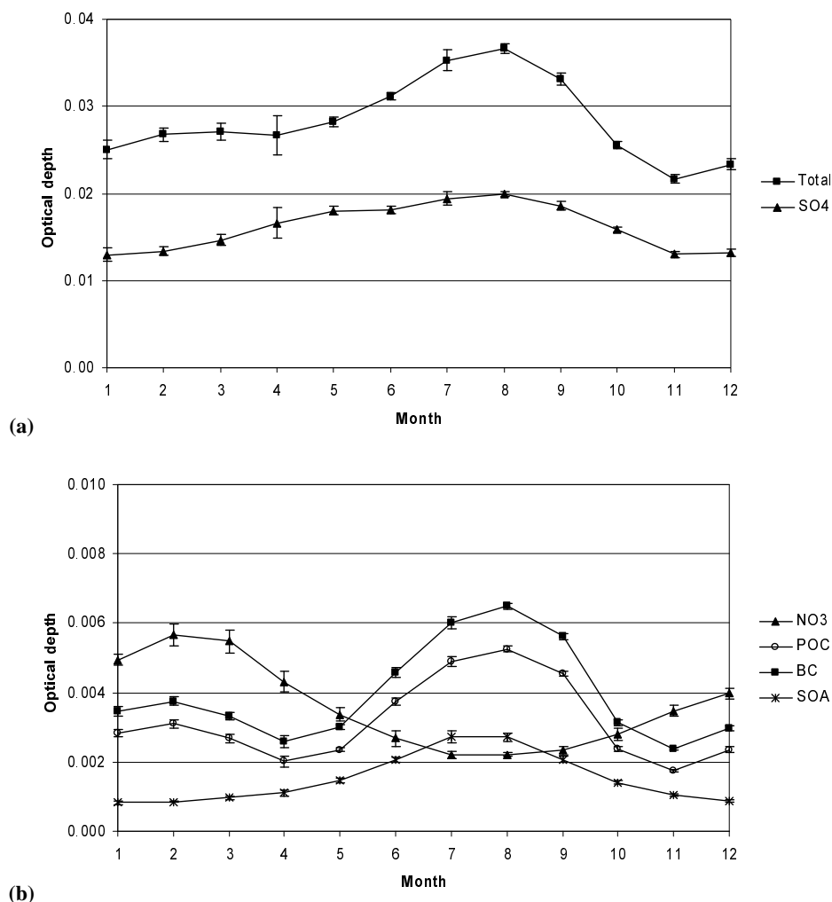
Fig. 10. Monthly mean average OD for the 10-year period of 1984–1993. (a) The error bars show the standard deviation of the interannual results. Total and \text{SO}_4 . (b) OD of other aerosol components.
