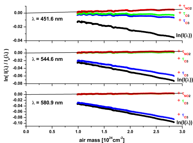
Fig. 2. Measured solar irradiance ratio ( \ln[E(\lambda)/E_o(\lambda)] ) for visible spectrometer at 3 wavelengths (upper panel: 451.6 nm, middle panel: 544.6 nm, lower panel: 580.9 nm) inferred for the Aire-sur-l'Adour/France measurement at \sim 32 km ( 83^\circ < SZA < 88^\circ ) on 9 October 2003. The data in black show the measured \ln[E(\lambda)/E_o(\lambda)] . The data in blue, green and red after accounting for Rayleigh scattering, O 3 absorption, and NO 2 absorption, respectively. The black lines show the regression to the Langley corrected data.
