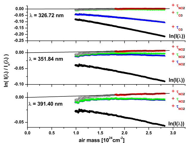
Fig. 1. Measured solar irradiance ratio ( \ln[E(\lambda)/E_o(\lambda)] ) for UV spectrometer at 3 wavelengths (upper panel: 326.7 nm, middle panel: 351.8 nm, lower panel: 391.4 nm) inferred for the Aire-sur-l'Adour/France measurement around \sim 32 km ( 83^\circ < SZA < 88^\circ ) on 9 October 2003. The data in black show the measured \ln[E(\lambda)/E_o(\lambda)] , the data in blue, green and red after accounting for Rayleigh scattering, O_3 absorption, and NO_2 absorption, respectively. The open grey data are discarded in the Langley regression (for details see text) and the black lines show the regression to the Langley corrected data.
