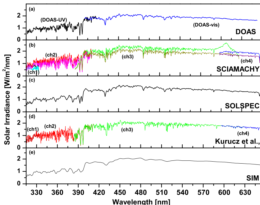
Fig. 3. Inter-comparison of measured solar irradiance spectra (a) for the DOAS measurements at Aire-sur-l'Adour at 32 km, on 9 October 2003; (b) for SCIAMACHY/ENVISAT in channel 1, 2, 3, and 4 using the present ESA SCIAMACHY calibration (upper curves) and the revised IUP-Bremen calibration (lower curves); (c) from SOLSPEC (Thuillier et al., 1997, 1998a, b); (d) from Kurucz et al. (1984) with recent updates of Fontenla et al. (1999) (MODTRAN 3.7) and convolved to the spectral resolution of SCIAMACHY in the respective channels; (e) from SORCE/SIM (Harder et al., 2000).
