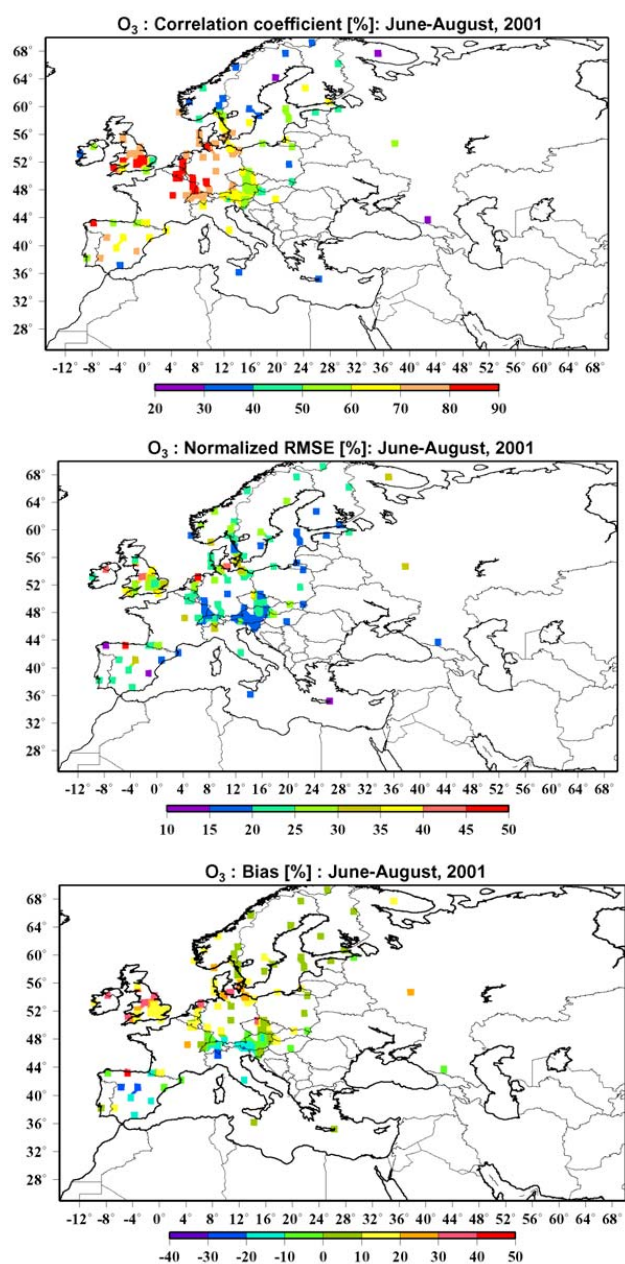
Fig. 2. Comparison statistics for daily maximums of ozone concentrations simulated by CHIMERE and measured by ground based ozone monitors.
