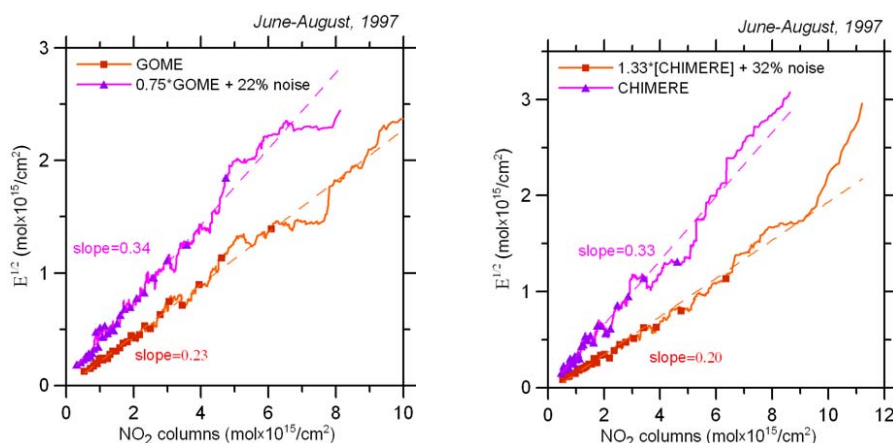
Fig. 8. The interpretation of the results presented in Fig. 7. The plots show the results of the same error analysis as in Fig. 7, but aimed at retrieving the known “errors” of the artificially transformed dataset. The “running window” analysis was applied to two pairs of the original and transformed datasets indicated in the figures, and the “running” RMSEs are plotted against the running averages of the indicated data.
