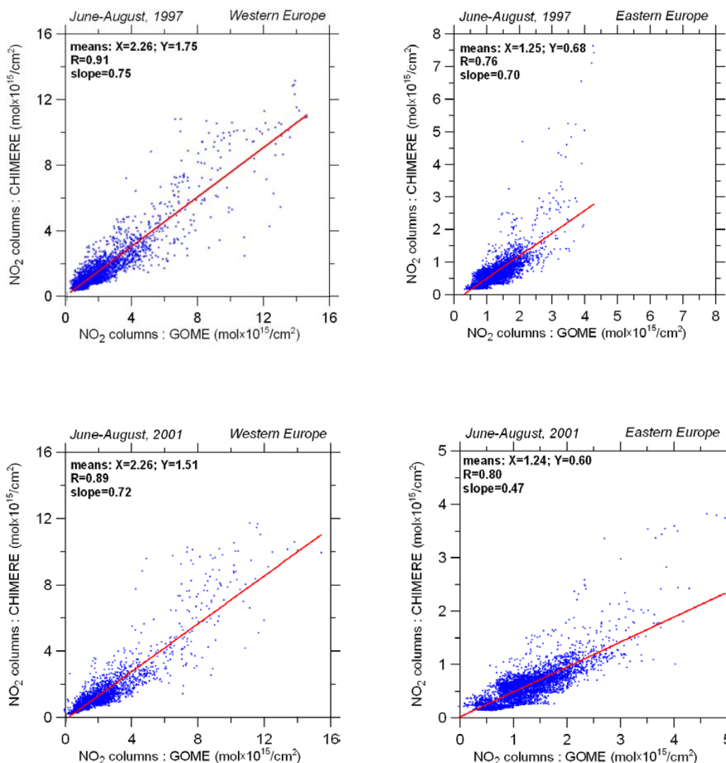
Fig. 6. Scatter plots of the simulated and GOME derived NO 2 columns for Western and Eastern Europe.
