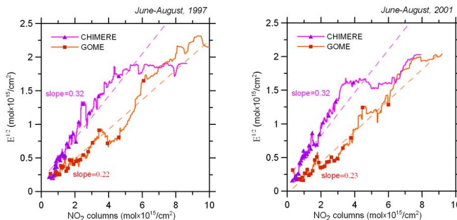
Fig. 7. Running averages of squared differences between the deviations of the simulated and GOME measurement derived tropospheric NO 2 columns from their running mean values versus the running averages of the indicated data for Western Europe. The averaging procedure using a running window covering 100 data points is applied to the gridded data for the seasonally averaged tropospheric NO 2 columns from GOME or CHIMERE (as indicated in the figures) arranged with growing amplitude. The points on the curves are depicted with a frequency of 1/100.
