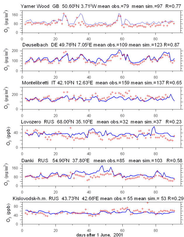
Fig. 3. Time series of daily maximums of ozone concentrations (mixing ratios) for summer season 2001. Solid lines and crosses show model results and observations, respectively. Note that the data are presented in original units of measurements for a given station.
