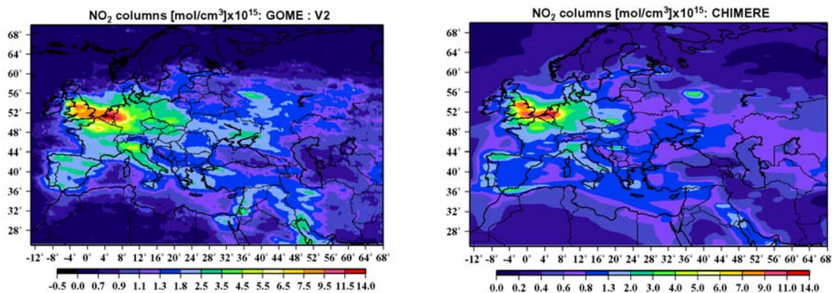
Fig. 5. Distributions of the tropospheric NO 2 columns derived from GOME measurements in comparison with the lower tropospheric NO 2 columns simulated by CHIMERE. The data shown represent the averages over summer months of 2001.
