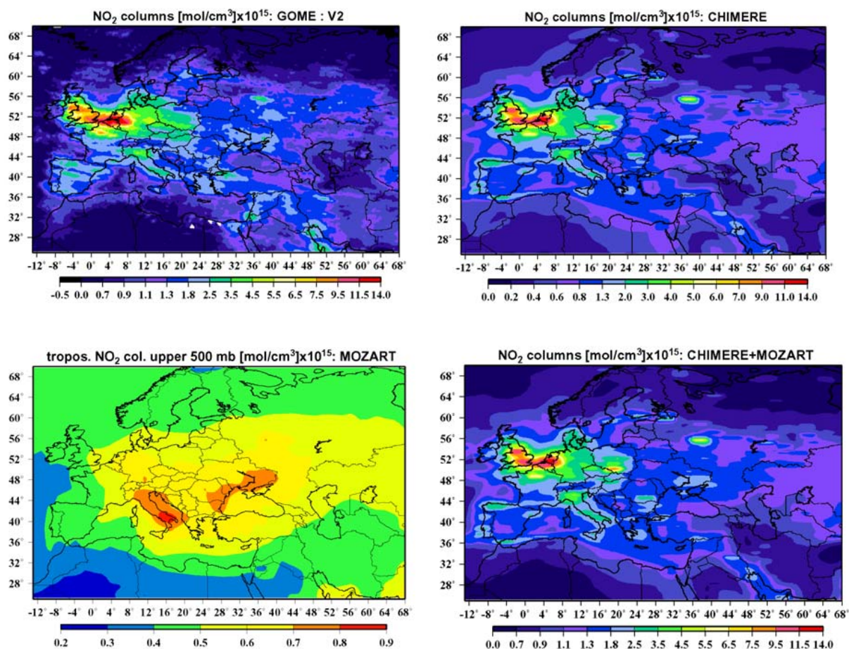
Fig. 4. Distributions of tropospheric NO 2 columns derived from GOME measurements in comparison with lower tropospheric NO 2 columns (above 500 hPa pressure level) simulated with CHIMERE, upper tropospheric NO 2 columns evaluated with MOZART, and composed (CHIMERE plus MOZART) total tropospheric NO 2 columns. The GOME and CHIMERE data represent the averages over the summer months of 1997. Upper tropospheric NO 2 were evaluated by averaging monthly NO 2 MOZART data corresponding to the summer of 1996. Note differences in scales of the plots.
