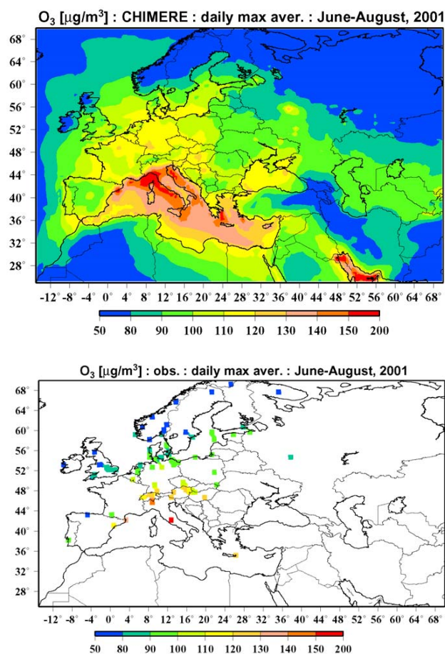
Fig. 1. Spatial distributions of daily maximum average ozone concentrations calculated by CHIMERE and observed at stations of the EMEP monitoring network.
