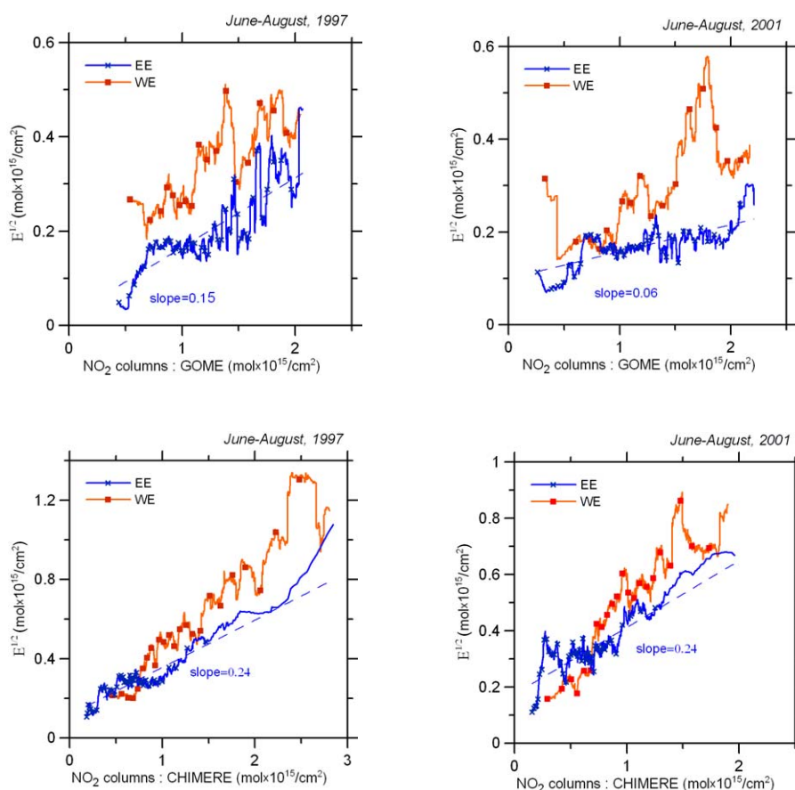
Fig. 9. The same as in Fig. 7, but for Eastern Europe. For convenience, the plots reproduce also a subsection of the dependences for Western Europe.
