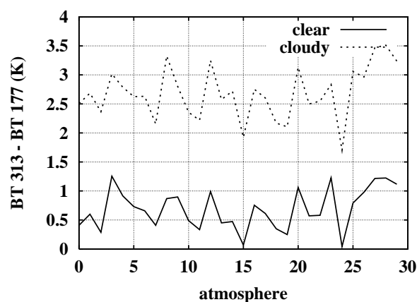
Fig. 2. Principle of cloud test: difference between channel 313 ( 3.83 \mu\text{m} ) brightness temperature and channel 177 ( 8.14 \mu\text{m} ) brightness temperature from radiative transfer simulations for 30 atmospheric tropical situations, for both clear and cloudy conditions. The threshold for this test is 1.5 K. The impact of dust on this difference is the opposite of the impact of clouds: it decreases BT 313–BT 177.
