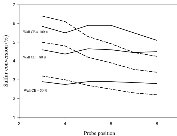
Fig. 3. Sulphur conversion factor \varepsilon required to obtain the same volatile particle concentrations as in DLR measurements, as a function of the probe position. Case of high FSC (1270 ppm). Dashed lines: old cruise. Solid lines: modern cruise. The agreement between observations and calculations is good for \varepsilon comprised between 2.5% and 6% approximately, whatever the collision efficiency CE used.
