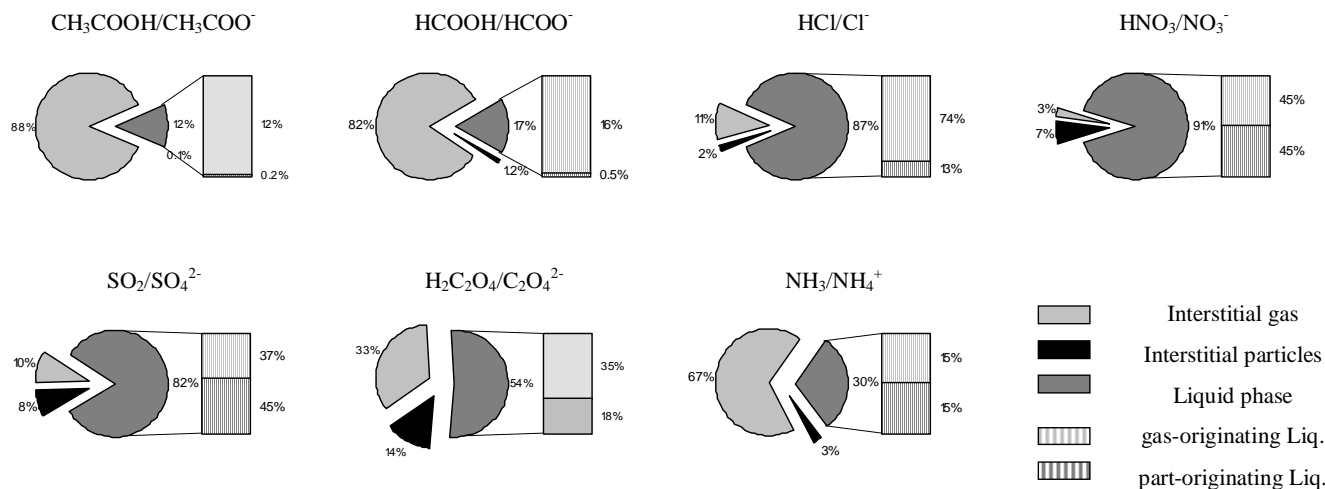
Fig. 2. Phase partitioning between the gas, particulate and liquid phases in cloud calculated from concentrations from the RJ1+Cascade Impactor (particulate), RJ1+Mist chambers (interstitial gas phase) and CDI (liquid phase). Further partitioning within the liquid phase between the gas-originating fraction and the particle-originating fraction are calculated from the CVI/CDI comparison. Gas concentrations are below detection limits for HCL, HNO 3 , SO 2 and H 2 C 2 O 4 , and thus their concentration are assimilated to detection limits.
