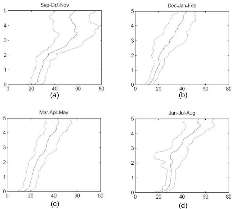
Fig. 6. Seasonal ozone profiles and standard deviation (ppbv) between 0 and 5 km derived from radiosondes at Runion (a) spring (SON) (b) summer (DJF) (c) autumn (MAM) (d) winter (JJA).
