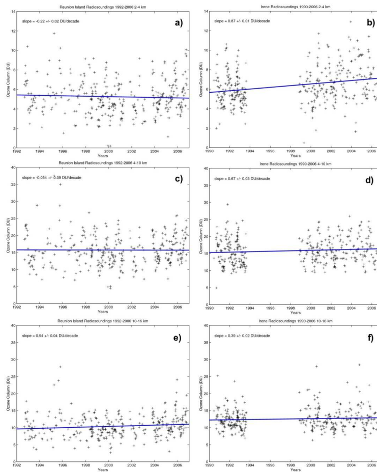
Fig. 8. Ozone trends between 2 and 4 km at Reunion ( a ) and Irene ( b ), between 4 and 10 km at Reunion ( c ) and Irene ( d ), and between 10 and 16 km at Reunion ( e ) and Irene ( f ).
