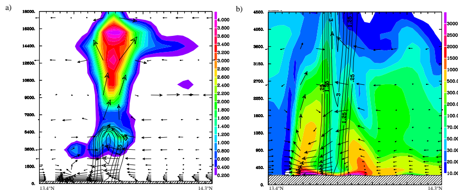
Fig. 15. Meridional cross section of the convective system (see location in Fig. 14) on 1 July 2006, 19:00 UTC. (a) Colored area represents the mixing ratio for cloud and ice ( \text{g kg}^{-1} ) and the isoline corresponds to the mixing ratio for rain ( \text{g kg}^{-1} ). (b) Colored area represents the dust concentration ( \mu\text{g m}^{-3} ) and the isoline corresponds to the mixing ratio for rain ( \text{g kg}^{-1} ). Vertical scales are not the same.
