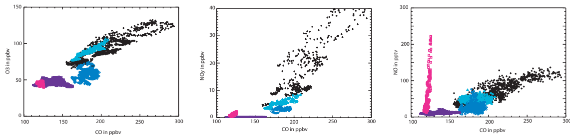
Fig. 2. Measured O_3 and reactive nitrogen concentrations ( NO, NO_y ) versus measured CO in the 5 Lagrangian match samplings. Black crosses represent measurements taken on 20 July and light blue triangles, dark blue diamonds, violet stars and pink squares the measurements taken on 21, 22, 25 and 26 July 2004, respectively.
