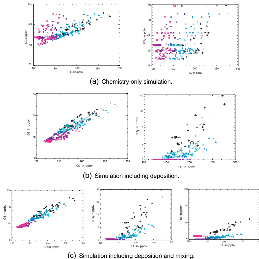
Fig. 9. Simulated concentrations of O_3 , NO_y and NO versus simulated CO concentrations in the 5 Lagrangian samplings. Black crosses represent measurement in the 20 July Lagrangian match and green triangles, blue diamonds, pink squares and violet stars show the simulated concentrations on 21, 22, 25 and 26 Lagrangian samplings, respectively.
