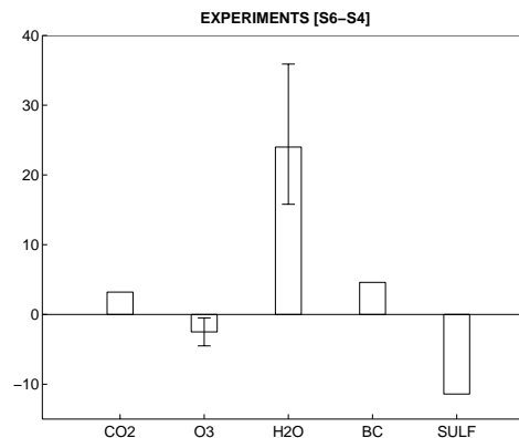
Fig. 7. Summary of (S6–S4) RF in year 2050, per component ( \text{mW/m}^2 ). \text{O}_3 and \text{H}_2\text{O} RF average values and variability are calculated using the DLR model radiative code applied to \text{O}_3 and \text{H}_2\text{O} changes (S6–S4) calculated by SLIMCAT, ULAQ-CTM, E39/C and OsloCTM2.
