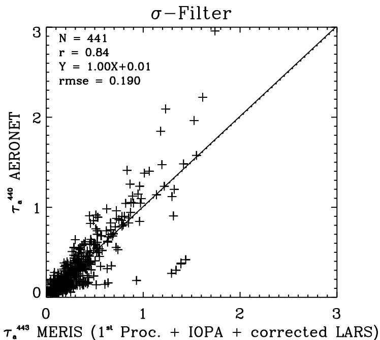
Fig. 13. Scatterplot of \tau_a AERONET versus 1st processing \tau_a MERIS retrieved with the IOPA models and the corrected LARS surface reflectance in the blue for the \sigma -filtered match-ups.
