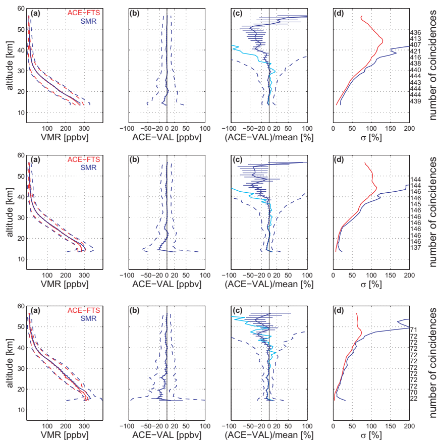
Fig. 2. Comparison of ACE-FTS and SMR N 2 O VMR profiles in five latitude bands. Top row: 60–90° N, middle row: 30–60° N, bottom row: 30° S–30° N. Panels (a), (b), (c) and (d) are the same as those in Fig. 1.
