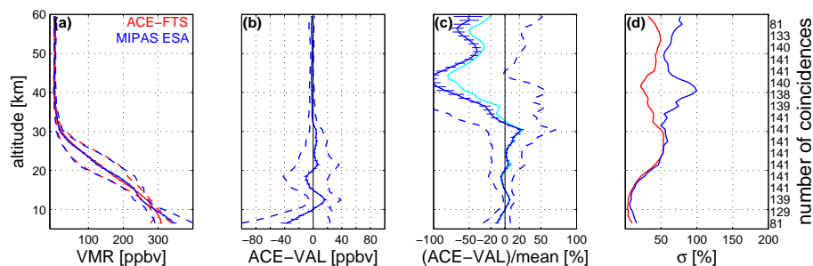
Fig. 5. Same as Fig. 1 but for comparisons between ACE-FTS and the MIPAS ESA N_2O data from 20–85° N.
