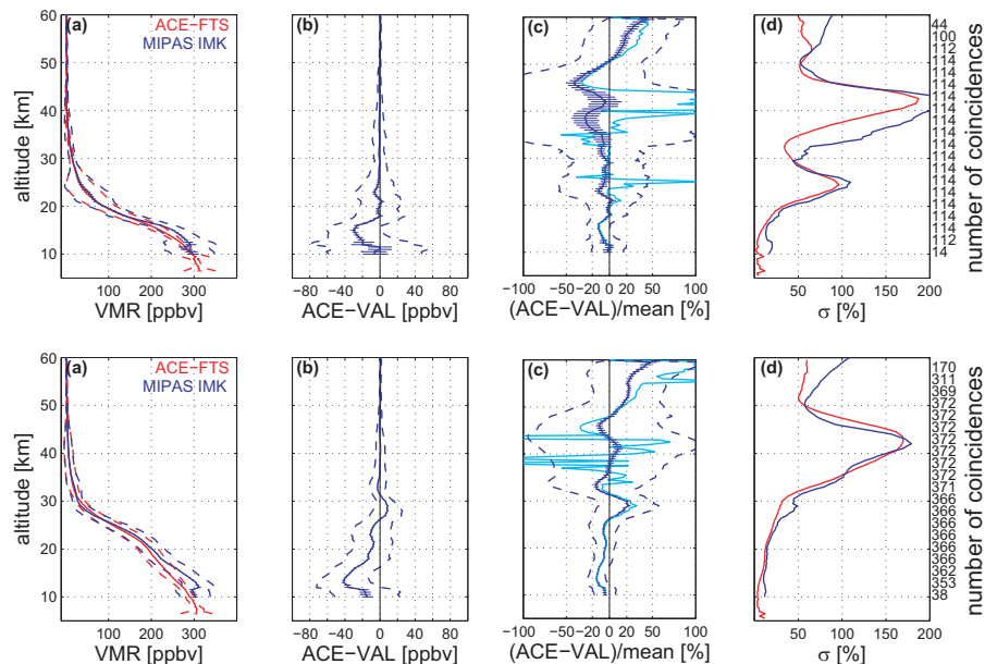
Fig. 6. Same as Fig. 1 but for comparisons between ACE-FTS and the MIPAS IMK-IAA \text{N}_2\text{O} data product for coincident measurements from 30–90° N inside (top row) and outside (bottom row) the polar vortex.
