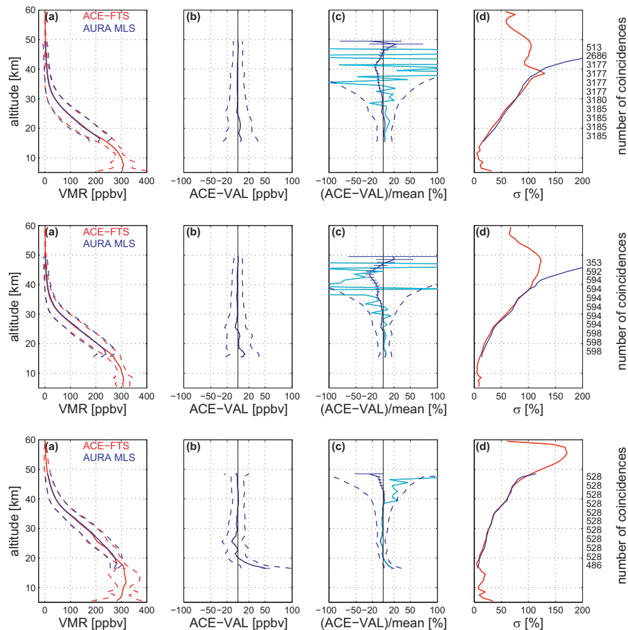
Fig. 4. Same as Fig. 2 but for comparisons between ACE-FTS and MLS. Top row: 60–90° N, middle row: 30–60° N, bottom row: 30° S–30° N.
