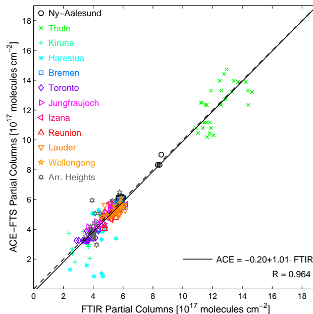
Fig. 11. Scatter plot of the ACE-FTS and ground-based FTIR \text{N}_2\text{O} partial columns shown in Fig. 10. The solid black line is the least-squares linear fit to the data, with the slope, intercept, and correlation coefficient given in the figure. The dotted line shows the one-to-one line relationship for comparison.
