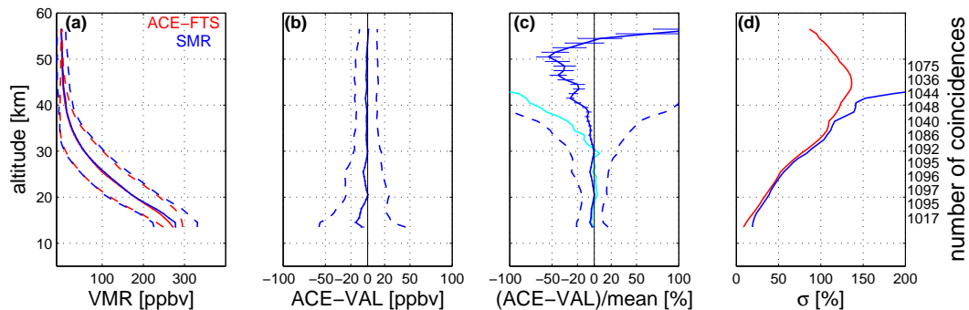
Fig. 1. Comparison of ACE-FTS and SMR \text{N}_2\text{O} VMR profiles from 90^\circ\text{S} – 90^\circ\text{N} . (a) Mean profiles for ACE-FTS (red solid line) and SMR (blue solid line). These mean profiles \pm 1\sigma standard deviation are plotted as dashed lines, and the standard errors in the mean ( \sigma/\sqrt{N} ) are included as error bars on the mean profiles. (b) Mean absolute difference profile (solid line) with \pm 1\sigma standard deviation (dashed lines) and the standard error in the mean (error bars). (c) Relative deviation from the mean, as a percentage, calculated using Eq. (3) (blue solid line) with \pm 1\sigma relative standard deviation (blue dashed lines) and the relative standard error in the mean (error bars). The profile of the mean relative difference calculated using Eq. (2) is also shown (cyan solid line). (d) Relative standard deviations on the mean profiles shown in (a). The number of coincident pairs at selected altitudes is given on the right-hand y-axis.
