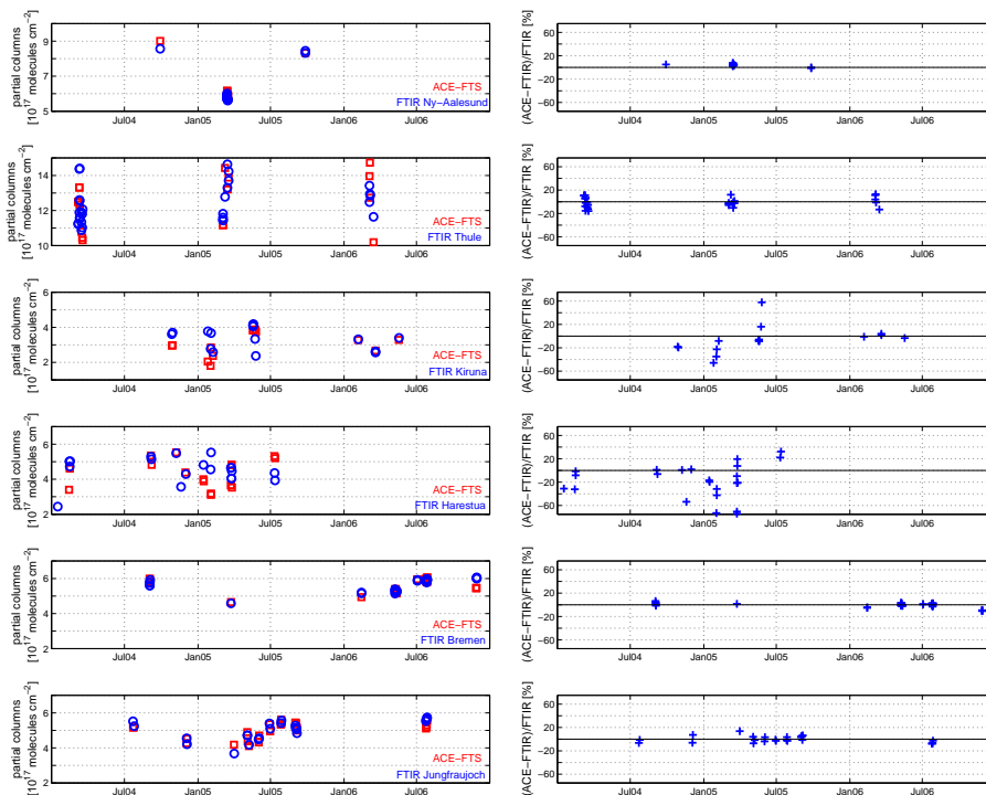
Fig. 10. Comparison of ACE-FTS and ground-based FTIR \text{N}_2\text{O} partial columns. For each station, the left-hand panel shows the time series of partial columns from ACE-FTS (red squares) and the FTIR (blue circles), and the right-hand panel shows the relative differences as a percentage of the FTIR partial columns. Note that the y-axis scales on the left-hand panels differ for some stations.
