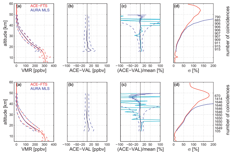
Fig. 4. Continued. Top row: 30–60° S, bottom row: 60–90° S.
