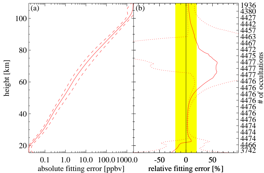
Fig. 3. Same as Fig. 1 but for ACE-FTS NO 2 .
