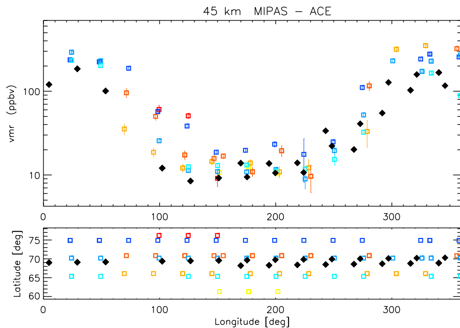
Fig. 31. Longitudinal distributions of ACE-FTS and MIPAS \text{NO}_x abundances measured on 18 March 2004 at VMR peak height (top) and respective geographic locations of the measurements (bottom). Black diamonds: ACE-FTS, open squares: MIPAS (color coding: yellow, orange, red: daytime measurements; green, blue: nighttime measurements).
