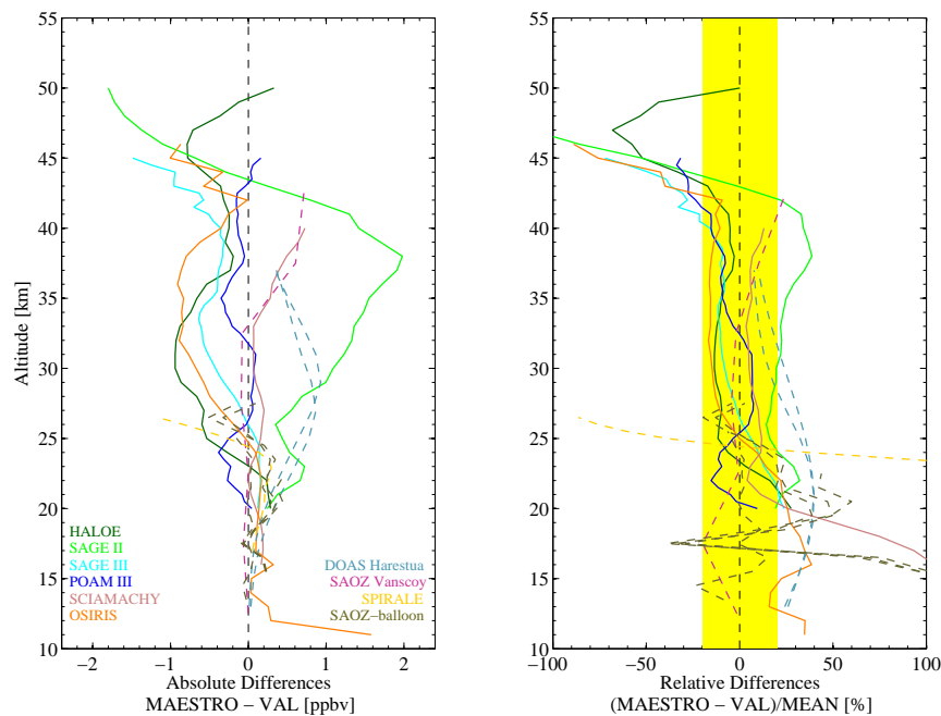
Fig. 39. Same as Fig. 38 but for MAESTRO. The SAGE III and POAM III results are taken from Kar et al. (2007). For SAGE II, results from the combined sunrise and sunset comparisons are shown.
