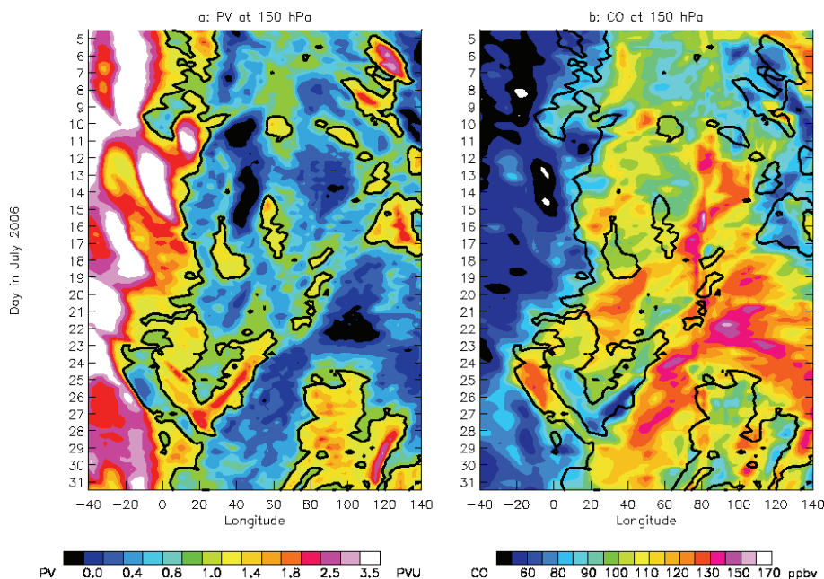
Fig. 8. Hovmoller diagrams of 6 h (a) PV and (b) CO assimilated mixing ratios at 150 hPa averaged over the latitudinal band 25°N–35°N for 5–31 July. The 1.2 PVU potential vorticity contour are represented as black solid lines.
