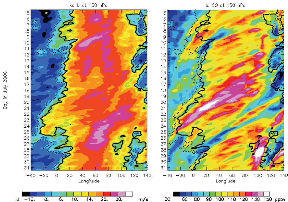
Fig. 9. Hovmöller diagrams of 6 h (a) zonal wind (greater than 0 for easterlies) and (b) CO assimilated mixing ratios at 150 hPa averaged over the latitudinal band 15° N–25° N for 5–31 July. Black solid lines: 10 m/s zonal wind, black dotted lines: 5 m/s zonal wind.
