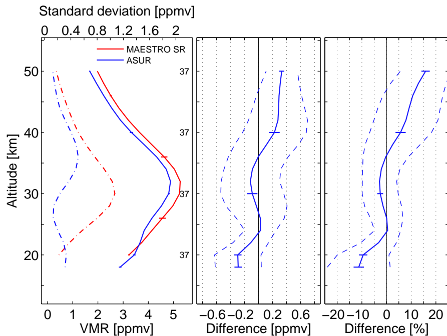
Fig. 25. Same as Fig. 2, but for the comparisons between ACE-MAESTRO and ASUR. Fractional differences are here expressed as (\text{ACE-MAESTRO} - \text{ASUR}) / \text{ACE-MAESTRO} [\%] .
