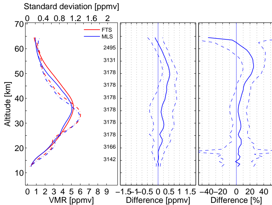
Fig. 22. Same as Fig. 8, but for the comparisons between ACE-FTS and Aura-MLS.
