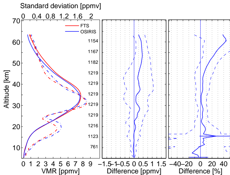
Fig. 9. Same as Fig. 8, but for the comparisons between ACE-FTS and OSIRIS (SaskMART).
