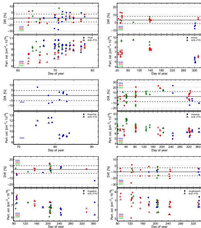
Fig. 40. Time series of ozone partial column comparisons for ACE-FTS with each ground-based FTIR instrument listed in Table 4. For each station, the bottom panel shows the partial column values for ACE-FTS (open triangles) and for the correlative FTIR measurements (filled diamonds). The top panel gives the relative differences between the partial column values for ACE-FTS and for the FTIR instruments, colour-coded according to the year of the observation: blue for 2004, red for 2005 and green for 2006. The horizontal black lines show the mean relative differences (solid) and the associated standard deviations (dashed). Note that the x- and y-axis scales used for each station are different.
