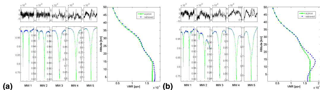
Fig. 6. Multiple micro-window fit of \text{CH}_4 plus interfering species from a single spectrum on (a) 16 October 2002 at Maïdo and on (b) 12 October 2004 at St-Denis. Measured (blue) and simulated spectra (green) are shown (left lower plot), together with the residuals (left upper plot), computed as measured minus simulated, and the a priori (green crosses) and retrieved profile (blue diamonds) (right plot).
