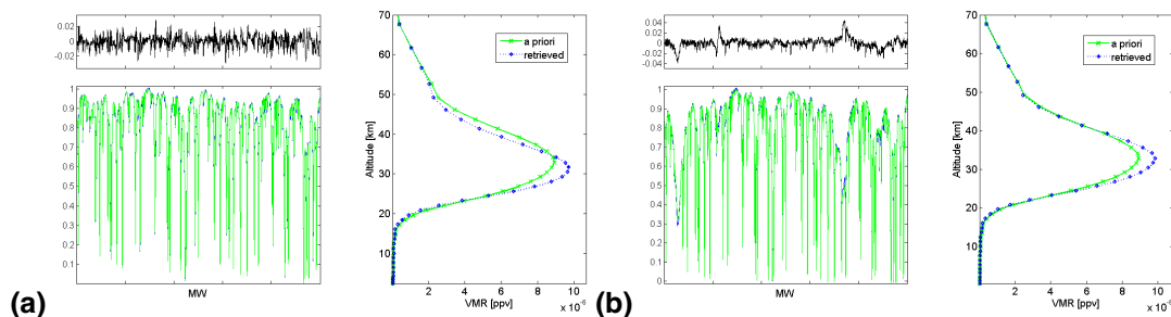
Fig. 5. Single micro-window fit of \text{O}_3 plus interfering species from a single spectrum on (a) 13 October 2002 at Maïdo and on (b) 15 October 2004 at St-Denis. Measured (blue) and simulated spectra (green) are shown (left lower plot), together with the residuals (left upper plot), computed as measured minus simulated, and the a priori (green crosses) and retrieved profile (blue diamonds) (right plot).
