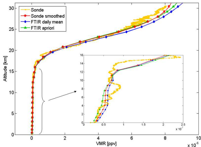
Fig. 17. Comparison of O_3 vertical profiles at St-Denis on 16 September 2004 obtained from ground-based FTIR (blue diamonds) and O_3 sonde (yellow dots). Green triangles indicate the a priori FTIR profile and red stars the sonde profile smoothed by the FTIR averaging kernels.
