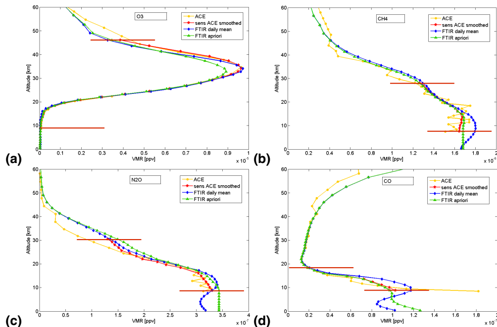
Fig. 18. Vertical vmr profiles from 0 to 60 km of (a) \text{O}_3 on 4 October, (b) \text{CH}_4 on 20 August, (c) \text{N}_2\text{O} on 4 October, (d) \text{CO} on 4 October, (e) \text{C}_2\text{H}_6 on 7 October, (f) \text{HCl} on 4 October, (g) \text{HF} on 20 August, and (h) \text{HNO}_3 on 20 August, measured at St-Denis in 2004 by ground-based FTIR (blue diamonds) and by ACE-FTS (raw: yellow circles; smoothed: red stars). The FTIR a priori profile is indicated by the green triangles.
