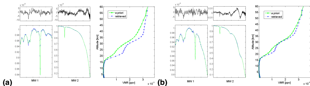
Fig. 14. Multiple micro-window fit of HCl plus interfering species from a single spectrum on (a) 16 October 2002 at Maïdo and on (b) 15 October 2004 at St-Denis. Measured (blue) and simulated spectra (green) are shown (left lower plot), together with the residuals (left upper plot), computed as measured minus simulated, and the a priori (green crosses) and retrieved profile (blue diamonds) (right plot).
