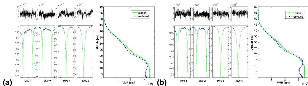
Fig. 7. Multiple micro-window fit of \text{N}_2\text{O} plus interfering species from a single spectrum on (a) 16 October 2002 at Maïdo and on (b) 12 October 2004 at St-Denis. Measured (blue) and simulated spectra (green) are shown (left lower plot), together with the residuals (left upper plot), computed as measured minus simulated, and the a priori (green crosses) and retrieved profile (blue diamonds) (right plot).
