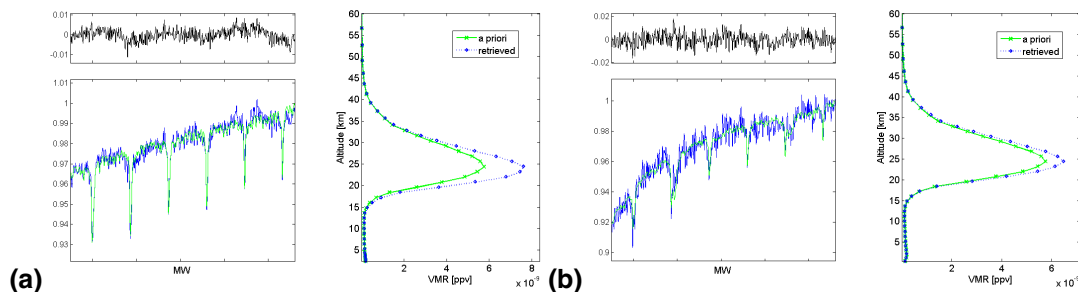
Fig. 16. Single micro-window fit of \text{HNO}_3 plus interfering species from a single spectrum on (a) 16 October 2002 at Maïdo and on (b) 21 October 2004 at St-Denis. Measured (blue) and simulated spectra (green) are shown (left lower plot), together with the residuals (left upper plot), computed as measured minus simulated, and the a priori (green crosses) and retrieved profile (blue diamonds) (right plot).
