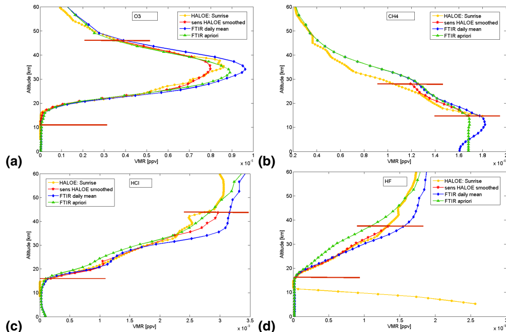
Fig. 19. Vertical vmr profiles from 0 to 60 km of (a) \text{O}_3 , (b) \text{CH}_4 , (c) \text{HCl} and (d) \text{HF} , measured at St-Denis by ground-based FTIR (blue diamonds) and by HALOE (raw: yellow circles; smoothed: red stars) on 16 September 2004. The green triangles indicate the a priori FTIR profile.
