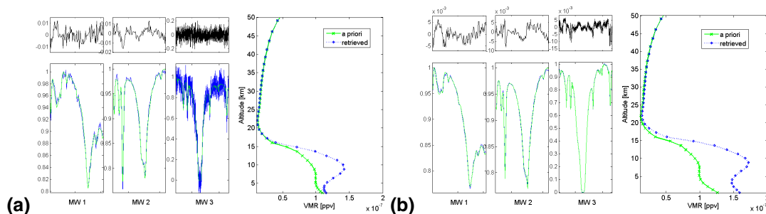
Fig. 8. Multiple micro-window fit of CO plus interfering species from a single spectrum on (a) 19 October 2002 at Maïdo and on (b) 12 October 2004 at St-Denis. Measured (blue) and simulated spectra (green) are shown (left lower plot), together with the residuals (left upper plot), computed as measured minus simulated, and the a priori (green crosses) and retrieved profile (blue diamonds) (right plot).
