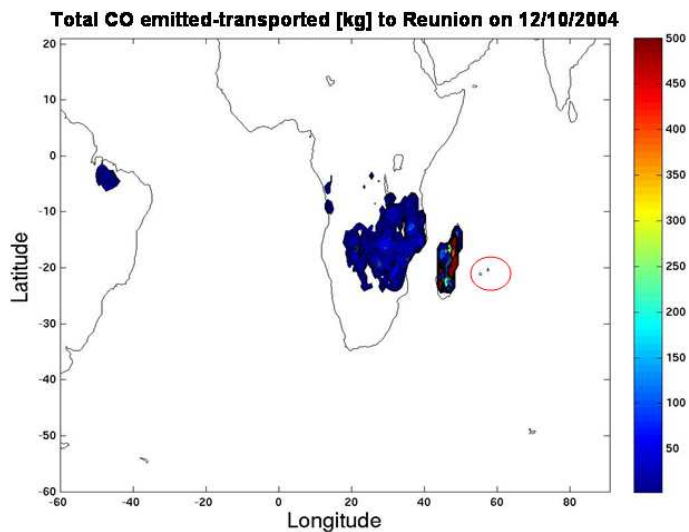
Fig. 11. Total amount of CO emitted and transported (in kg) to Ile de La Réunion (located within the red circle) on 12 October 2004, calculated by FLEXPART.
