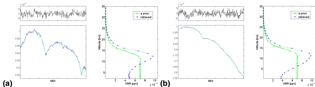
Fig. 12. Single micro-window fit of C_2H_6 plus interfering species from a single spectrum on (a) 14 October 2002 at Maïdo and on (b) 9 October 2004 at St-Denis. Measured (blue) and simulated spectra (green) are shown (left lower plot), together with the residuals (left upper plot), computed as measured minus simulated, and the a priori (green crosses) and retrieved profile (blue diamonds) (right plot).
