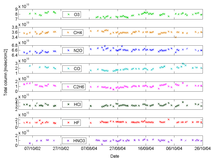
Fig. 4. Time series of the total column amounts (in molecules/cm 2 ) at St-Denis in 2002 and 2004 for all retrieved species.
