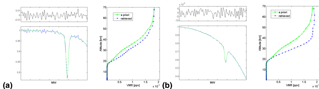
Fig. 15. Single micro-window fit of HF plus interfering species from a single spectrum on (a) 13 October 2002 at Maïdo and on (b) 11 October 2004 at St-Denis. Measured (blue) and simulated spectra (green) are shown (left lower plot), together with the residuals (left upper plot), computed as measured minus simulated, and the a priori (green crosses) and retrieved profile (blue diamonds) (right plot).
