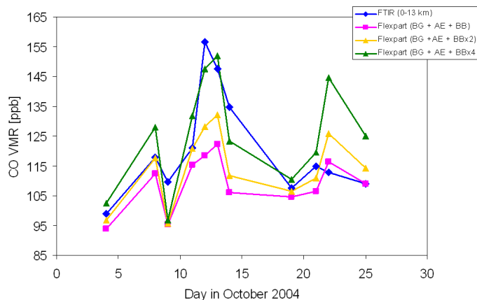
Fig. 10. Time series of CO abundances at St-Denis between 0 and 13 km, in October 2004, calculated by ground-based FTIR (blue diamonds) and FLEXPART with (1) GFED emissions (pink squares), (2) GFED emissions \times 2 (yellow triangles), (3) GFED emissions \times 4 (green triangles).
