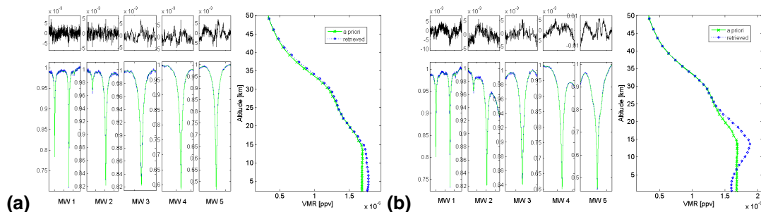
Fig. 6. Multiple micro-window fit of \text{CH}_4 plus interfering species from a single spectrum on (a) 16 October 2002 at Maïdo and on (b) 12 October 2004 at St-Denis. Measured (blue) and simulated spectra (green) are shown (left lower plot), together with the residuals (left upper plot), computed as measured minus simulated, and the a priori (green crosses) and retrieved profile (blue diamonds) (right plot).
