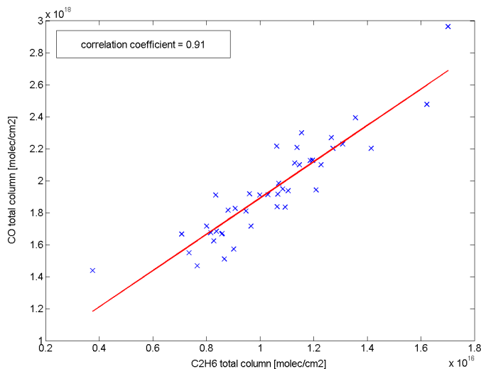
Fig. 13. Correlation plot of CO versus C 2 H 6 total column amounts (in molecules/cm 2 ) during the FTIR campaigns at St-Denis in 2002 and 2004.
