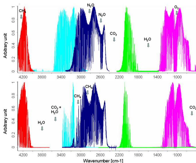
Fig. 1. Composite spectra for different bandpass filters (NDSC-1: red, NDSC-2: blue, NDSC-3: dark blue, NDSC-5: green, and NDSC-6: pink), taken at Maïdo (upper plot) and at St-Denis (bottom plot) in 2002, for solar zenith angles between 40° and 50°.
