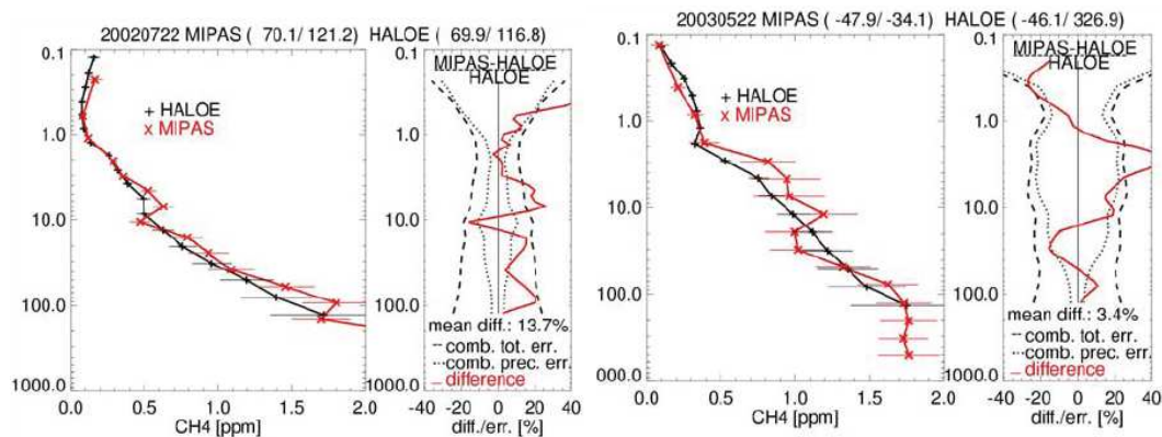
Fig. 18. Comparison between individual HALOE and MIPAS profiles in two different geographical regions (Arctic and southern mid-latitudes).
