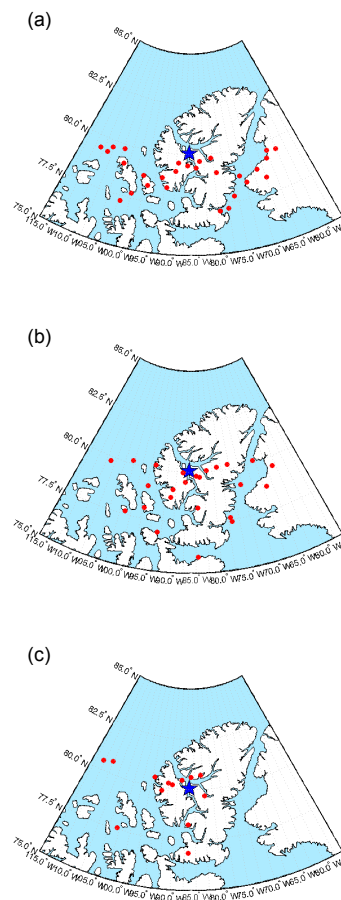
Fig. 2. Location of ACE occultations at 30 km altitude within 500 km of PEARL in February and March (a) 2004, (b) 2005, and (c) 2006. The blue star indicates the location of PEARL.
