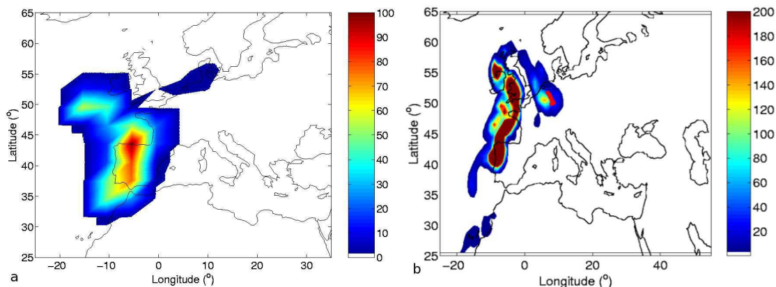
Fig. 10. (a) FLEXPART CO fire plume (ppbv) horizontal section at 2.5 km altitude on 6 August 2003 at the time of the MOZIAIC profile shown on Fig. 9. The MOZIAIC aircraft path around 2.5 km altitude is superposed in red. (b) Emission sensitivity distribution in the 0–3 km column for trajectory particles arriving along the MOZIAIC profile displayed on Fig. 9. Particles were released only where the measured CO exceeded 150 ppbv. Residence times were calculated from arrival until 3 days back and values are given as percentage of the maximum.
