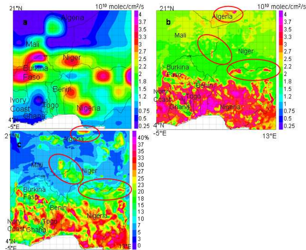
Fig. 2. (a) Biogenic NO emissions from soil ( 10^{10} \text{ molec.cm}^{-2}.\text{s}^{-1} ) in August, provided by GEIA database, from Yienger and Levy (1995) inventory, (b) biogenic emissions from soils ( 10^{10} \text{ molec.cm}^{-2}.\text{s}^{-1} ) provided by the on line ANN algorithm, 6 August 2006 15:00 UTC, and (c) soil moisture (%), 6 August 2006 15:00 UTC. Red circles highlight the correspondence between strong moisture and high emissions.
