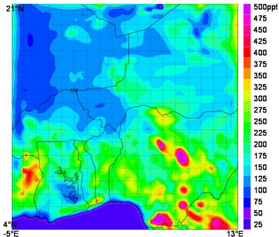
Fig. 9. \text{NO}_x concentrations in ppt, at 200-m height above ground level (corresponds to 450 m above sea level in the region of Niamey), from ALLNOX simulation at 15:00 UTC, 6 August.
