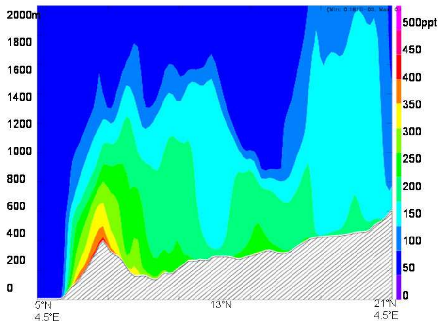
Fig. 8. Vertical cut of \text{NO}_x concentrations in ppt ( 4.5^\circ\text{E} , from 5 to 21^\circ\text{N} ), ALLNOX simulation, from 0 to 2000\text{ m} . 6\text{ August }2006, 15:00\text{ UTC}
