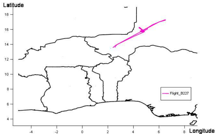
Fig. 6. The track (latitude vs. longitude) of flight B227 of the BAe-146, 6 August 2006.
