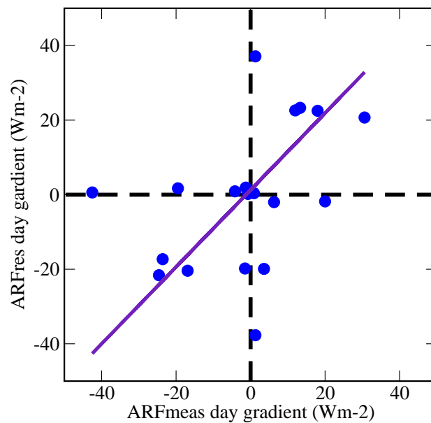
Fig. 9. Temporal gradient of ARF over one day in Palaiseau and Carpentras. Satellite based method against ground-based measurement estimate. Linear regression is also plotted.
