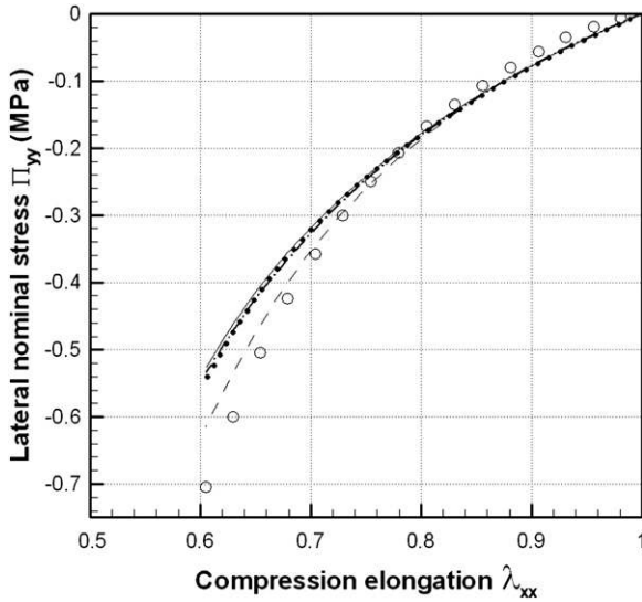
Fig. 11. Experimental data (○) and model predictions ((- -) Mooney, (- · -) Gent, (· · ·) Haines and Wilson and (—) Ogden) for the lateral stress during the plane strain compression test.
