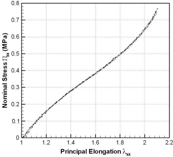
Fig. 5. Tensile test: two load/unload cycles performed at two elongation rates: (—) 2 \cdot 10^{-4} \text{ s}^{-1} and (- -) 10^{-1} \text{ s}^{-1} .
