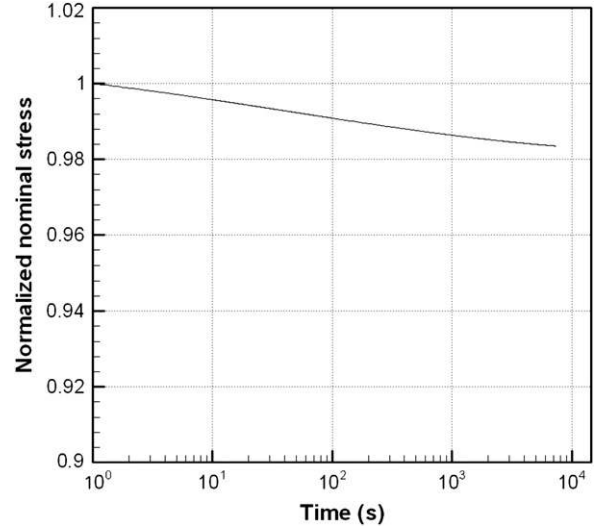
Fig. 6. Time evolution of the normalised stress \Pi_{xx}/\Pi_{xx}(t = t_0) , for a stress relaxation test recorded after a monotonic tensile test performed at \lambda=2 .
