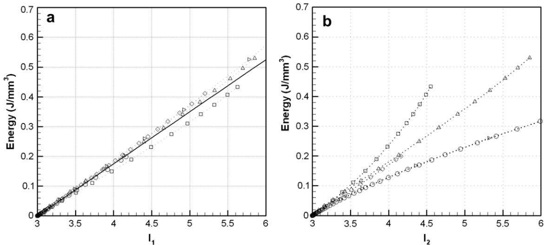
Fig. 8. Evolution of the elastic energy density as a function of (a) I_1 and (b) I_2 for the five homogeneous tests performed for fit: ( \square ) uniaxial tensile, ( \Delta ) pure shear, ( \circ ) simple compression, ( \diamond ) plane strain compression and ( \triangleright ) bulge test. The fitted neo-hookean model is also represented (—).
