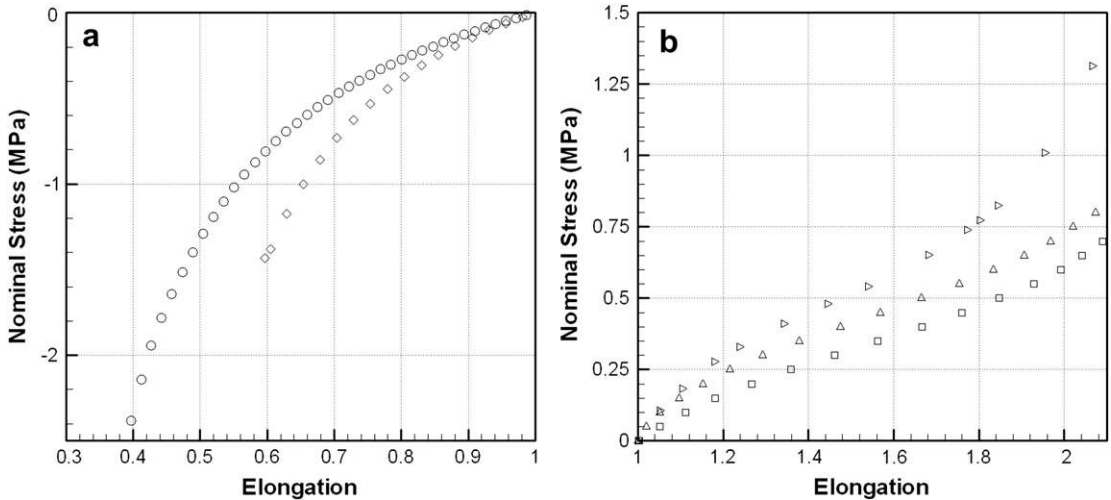
Fig. 7. Principal stress–elongation curves obtained in: (a) (○) simple compression, (◇) plane strain compression; (b) (□) uniaxial tensile, (△) pure shear and (▷) bulge tests.
