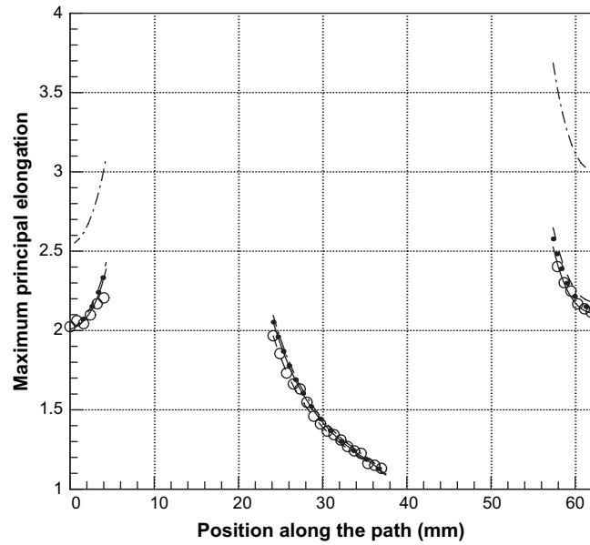
Fig. 15. Experimental and simulated elongations along the path defined in Fig. 14 at 20 N: (○) experimental data, (·-·) Mooney, (- -) Gent, (···) Haines and Wilson and (—) Ogden; the blank in the curves are due to the holes.
