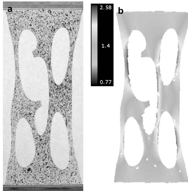
Fig. 12. Photograph of the deformed plate for an applied force of 20 N: (a) deformation of the pattern, (b) colour map: major principal elongation (result of 7D).
