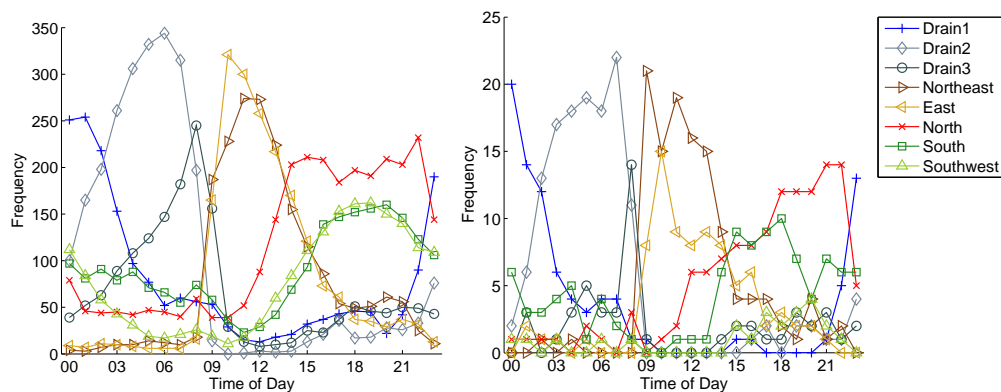
Fig. 8. Histogram of the diurnal distribution of the surface wind clusters (Sfc c ) for the 10 year record (left) and the MILAGRO field campaign (right).
