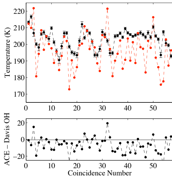
Fig. 6. A comparison of 57 coincident Davis OH rotational temperatures (black) with ACE-FTS v2.2 temperatures (red) at 87.5 km altitude (top) and differences (bottom; in K). The error bars on the OH rotational temperature time series are 1\sigma standard deviation in the nightly mean.
