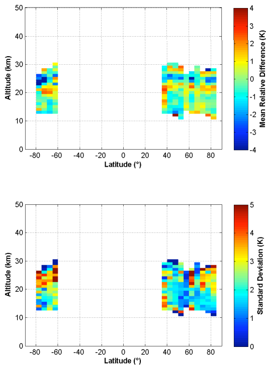
Fig. 21. Mean relative differences between ACE-FTS and radiosonde data versus altitude and latitude (top) and corresponding standard deviation (bottom) averaged in 5^\circ latitude bins.
