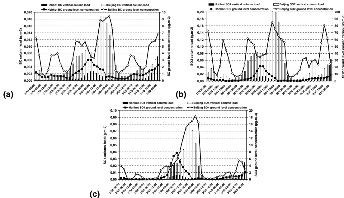
Fig. 13. Time series, since 27 April, 00:00 UTC, to 2 May, 00:00 UTC, 2005, of modelled surface concentration ( \mu\text{g m}^{-3} : specific scale on the right, for each specie) and of column load ( \text{g m}^{-2} : specific scale on the left, for each specie), at Hohhot (black squares and bar charts) and Beijing (white diamonds and bar charts), for the three anthropogenic species: BC (a) , \text{SO}_2 (b) and Sulphates (c) .
