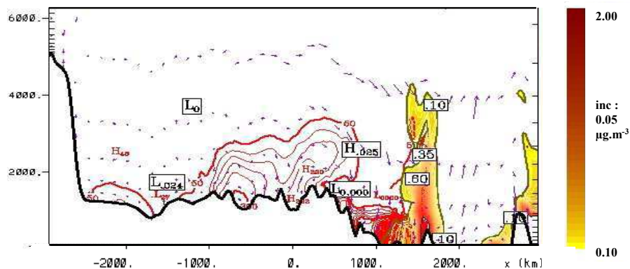
Fig. 8b. Isocontours of vertical “captured” \text{SO}_2 concentrations and of vertical mineral dust concentrations as Fig. 8a, but with vertical zonal cross-section (along pink line of Fig. 8a).
