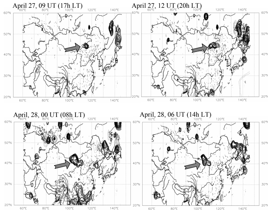
Fig. 6a. Changes of relative visibilities interpolated in Asia for 27 April and 28 April 2005. Thick lines: decreasing of more than 50%; Thin lines: rainfall (arbitrary units); Thin dotted lines: RH > 80\% (a.u.); vectors: wind (a.u.); large arrows locate the main area of interest.
