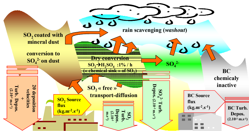
Fig. 3. Processes for sulphur compounds, mineral dust and BC used in the simplified model of transports and captures.
