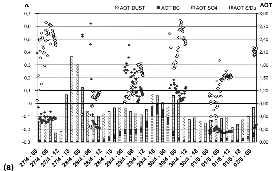
Fig. 14. Time series, since 27 April, 00:00 UTC, to 2 May, 00:00 UTC, 2005, of modelled AOT, with respective AOT contributions of mineral dust (light grey columns with points, top of total columns if present), BC (dark grey columns), \text{SO}_4^{2-} (horizontal grey and white stripes) and “captured” \text{SO}_2 (vertical stripes, far from visible on the 3 sites of China/Mongolia). Also displayed: AERONET AOT (black diamonds, right scale, common to the modelled AOT) and Angstrom Exponent \alpha (white diamonds, left scale). Results for Beijing (China a ), Dalanzadgad (Mongolia b ), Liangning (China, c ), Gwangju (Korea, d ) and Osaka (Japan, e ), with specific scales for each site.
