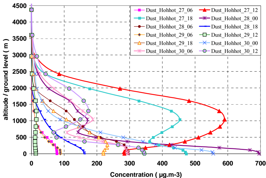
Fig. 11a. Time vertical profiles of dust concentrations ( \mu\text{g m}^{-3} ), between surface and 4500 m above Hohhot (UTC hours).
