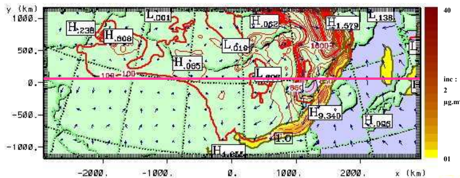
Fig. 8a. Isocontours of surface “captured” \text{SO}_2 concentrations ( \mu\text{g m}^{-3} , yellow-coloured and black labels: H means maximum and L means minimum) and of surface mineral dust concentrations (red-coloured and labels). Blue arrows: surface winds (a.u.). Model results at 00:00 UTC (08:00 LT) for 1 May 2005.
