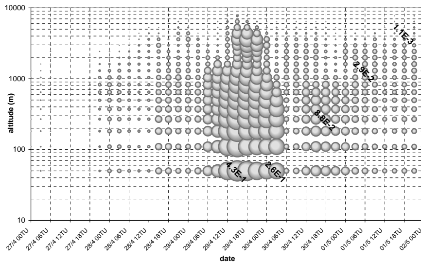
Fig. 9. Symbolic intercomparison of the “captured” SO 2 concentrations (grey spheres): time series (UTC) of the vertical distributions (altitudes: logarithmic scale) above Beijing.
