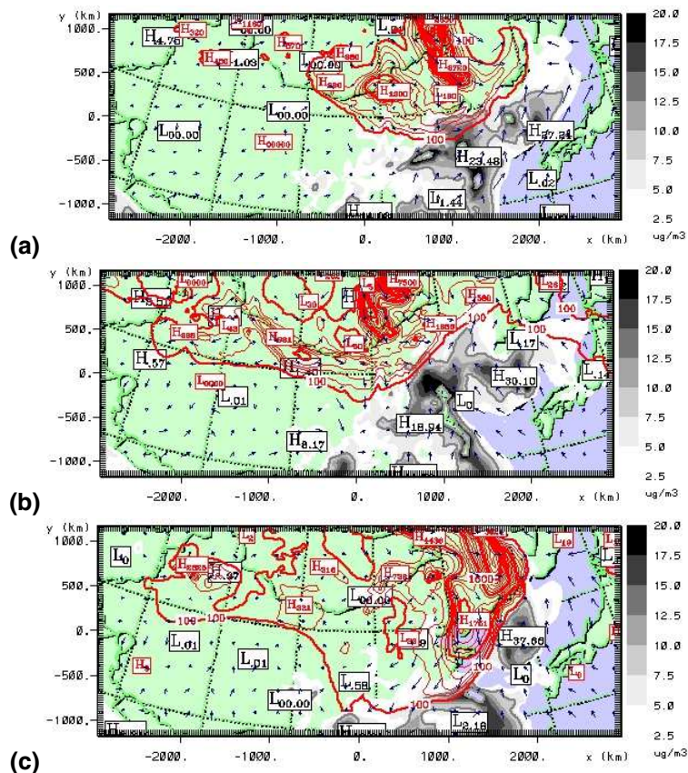
Fig. 7. Isocontours of surface BC concentrations ( \mu\text{g m}^{-3} , grey-coloured and black labels: H means maximum and L means minimum) and of surface mineral dust concentrations (red-coloured and labels). Blue arrows: surface winds (a.u.). Model results at 00:00 UTC (08:00 LT) on 28 April (a), 30 April (b) and 1 May (c), 2005.
