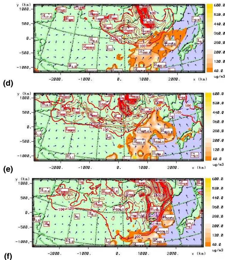
Fig. 7. Isocontours of surface \text{SO}_2 concentrations ( \mu\text{g m}^{-3} , orange-coloured and brown labels: H means maximum and L means minimum) and of surface mineral dust concentrations (red-coloured and labels). Blue arrows: surface winds (a.u.). Model results at 00:00 UTC (08:00 LT) on 28 April (d), 30 April (e) and May 1 (f), 2005.
