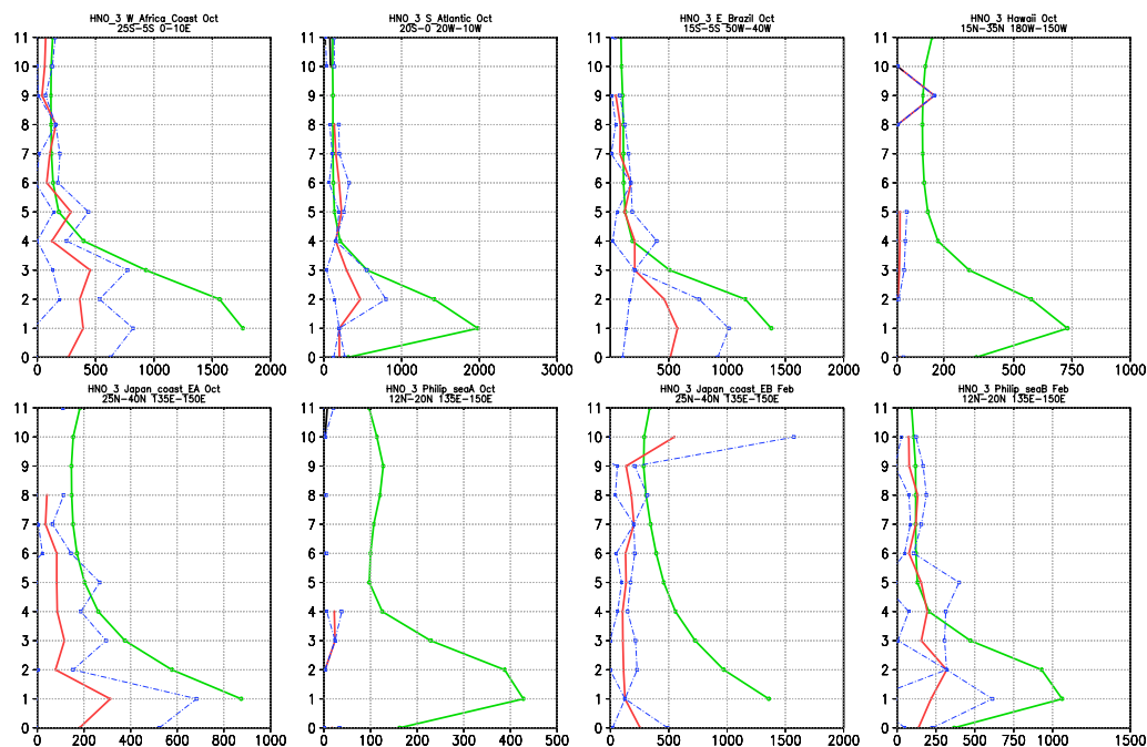
Fig. 12. MOCAGE-Climat T42 mean vertical profiles of HNO 3 mixing ratios (pptv, in green) against aircraft field campaign observations (Emmons et al., 2000). Regions of the world are as presented in Horowitz et al. (2003); vertical is between the surface and 11 km. The observations are shown as mean (red lines), ±2 standard deviations (blue dotted lines).
