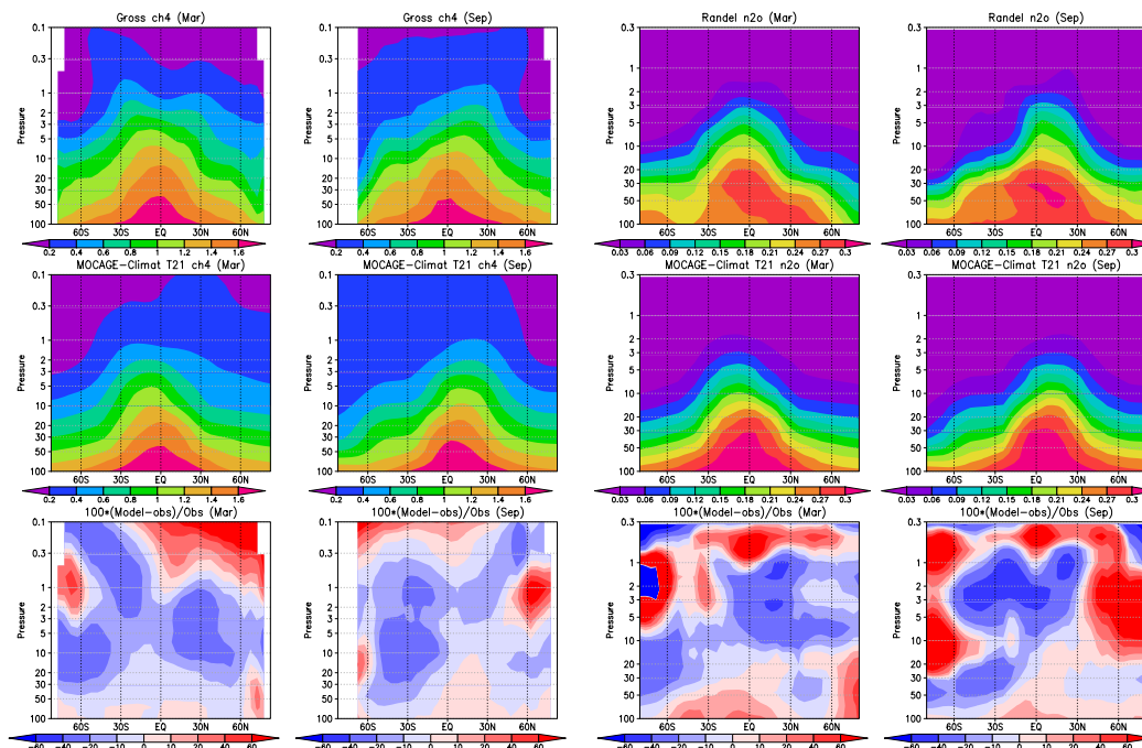
Fig. 3. First two columns: MOCAGE-Climat T21 zonal monthly mixing ratios of CH 4 (ppmv) against the Gross and Russel (2005) climatology, and relative differences ( 100 \times (\text{Model} - \text{Obs}) / \text{Obs} ), between 100 and 0.1 hPa, in March (left panels) and September (right panels). Last two columns: MOCAGE-Climat T21 zonal monthly mixing ratios of N 2 O (ppmv) against the Randel et al. (1998) climatology, and relative differences ( 100 \times (\text{Model} - \text{Obs}) / \text{Obs} ), between 100 and 0.3 hPa, in March (left panels) and September (right panels).
