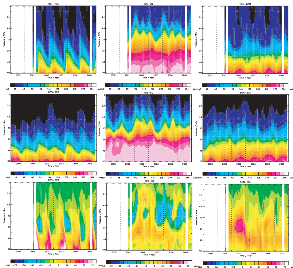
Fig. 7. Time/pressure series for N 2 O zonally averaged bands of 10 degrees, 80 S–70 S (left panels), 10 S-EQ (middle panels) and 50 N–60 N (right panels), for ODIN observations (upper line, in white no observations), simulated by MOCAGE-Climat (middle line) and absolute differences (model - observations) (ppbv) (bottom line).
