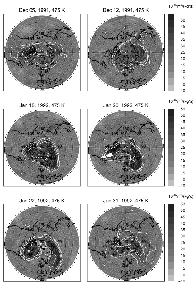
Fig. 4. Potential vorticity derived from MetO analysis on the 475 K potential temperature level valid for 5, 12 December 1991, and 18, 20, 22 and 31 January 1992, 12:00 UTC. White lines indicate the location of the polar vortex core, edge, and outer edge of the vortex as defined by Nash et al. (1996). The location of Kiruna is marked as a white diamond. For the same altitude the location of ER-2 aircraft measurements are presented as white triangles for 20 January, only (taken within 8 hr at the day shown).
