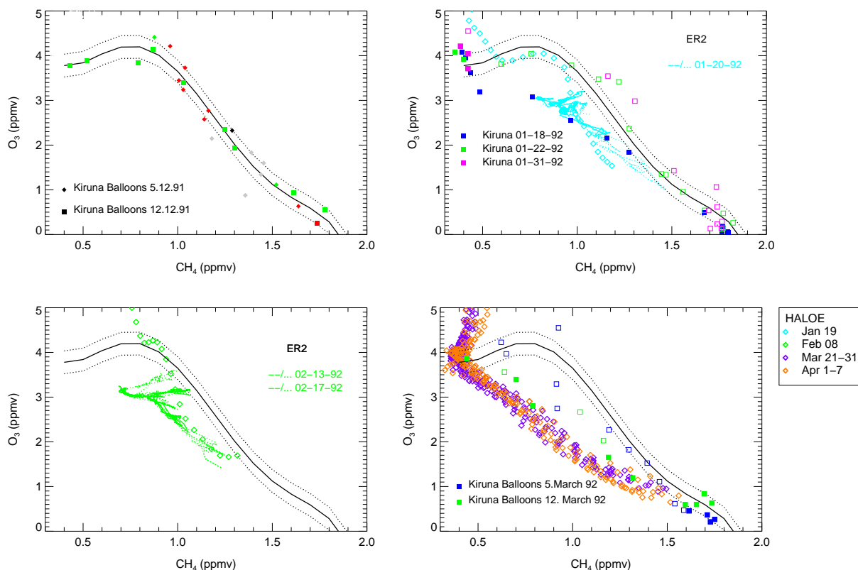
Fig. 6. O_3/CH_4 relations, the early winter reference function, shown as a black line in all four panels, was derived using Kiruna balloon data from 5 and 12 December 1991 (top left panel). Different colors indicate the position of the data, vortex core (green), entire vortex (red), vortex boundary region (black) and outside the vortex (grey). Top right panel: O_3/CH_4 relations during January 1992 using ER-2 aircraft measurements within the entire vortex (cyan dotted lines) and within the vortex core (cyan solid lines), Kiruna balloon data within the vortex core (filled colored squares) and outside the vortex core (open colored squares) and HALOE satellite observations (cyan diamonds) within the polar vortex. Bottom panel: O_3/CH_4 relations during February (right panel) and March / April (left) in 1992 using ER-2 available aircraft measurements within the vortex (green lines) and HALOE satellite observations (colored diamonds) within the polar vortex.
