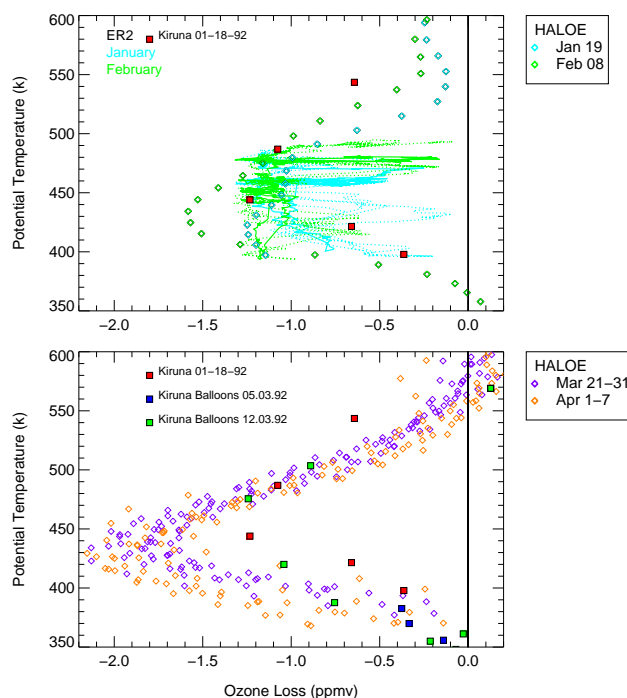
Fig. 7. Ozone loss profiles derived from O_3/CH_4 tracer relations between mid-December 1991 and January/February 1992 (top panel) and mid-December and March/April (bottom panel). HALOE and balloon data observed in the vortex core are shown, as well as ER-2 aircraft data in the entire vortex (dotted lines) and in the vortex core (solid lines).
