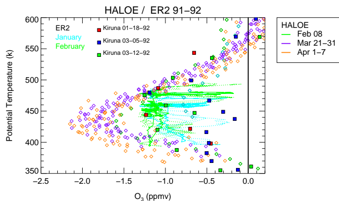
Fig. 6. Ozone loss profiles derived from O 3 /CH 4 tracer relations between January und April (see text).
