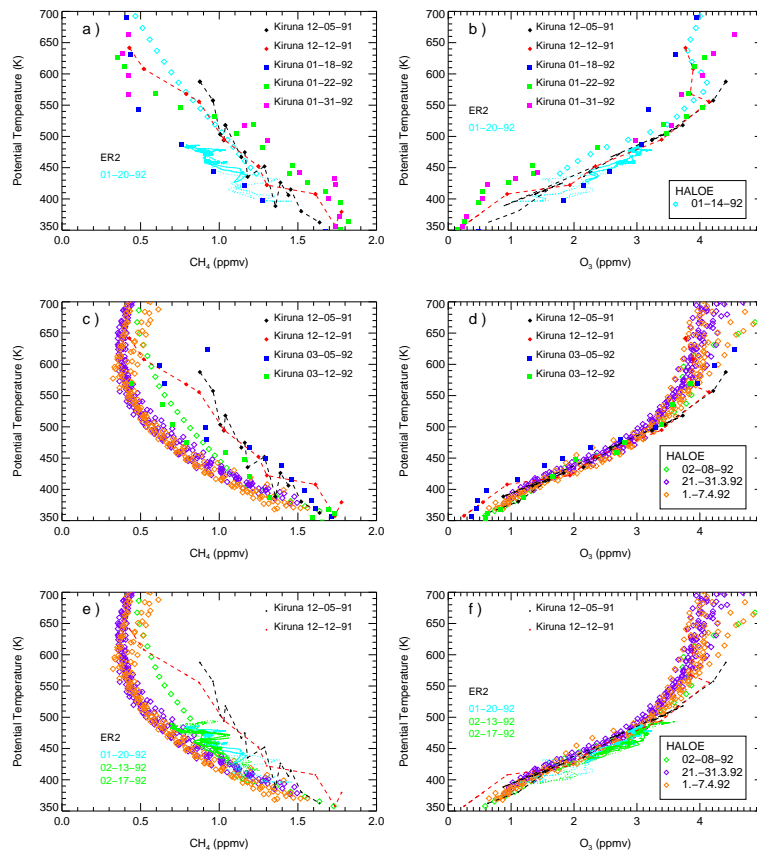
Fig. 2. CH 4 (left column) and O 3 (right column) mixing ratios with respect to potential temperature taken by the HALOE satellite, Kiruna balloons and ER-2 aircraft observations within the vortex core (solid lines) and within the entire vortex (dotted lines), for different periods (see text). Kiruna balloon observations during December (red and black symbols and dashed lines) are shown in each panel as early winter reference profiles.
