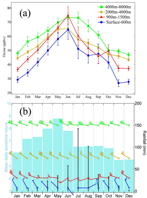
Fig. 6. Seasonal variations of (a) O 3 concentrations at different tropospheric levels over Beijing, and of (b) wind profiles, mean sunshine hours and monthly total rainfall at Beijing.
