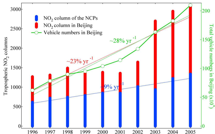
Fig. 13. Trends of annual mean tropospheric NO 2 columns (Unit: 1e^{13} molecules/cm 2 ) in the NCPs and Beijing (data from GOME and SCIAMACHY), and annual total numbers of civilian vehicles in Beijing (Data from Chinese Statistical Yearbook 1996–2006).
