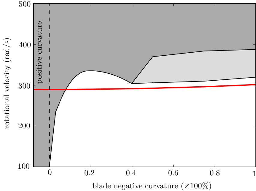
Figure 21: The different possible vibratory behaviors of the structures are given with respect to the blades curvature and the rotational velocity; N = 22 , k = 3 and \mu = 1 ; damped, sustained, divergent, and — analytical solution.
