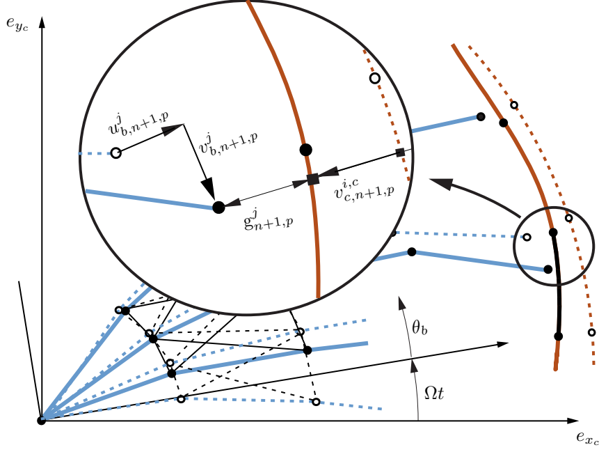
Figure 7: Initial (----) and current predicted (—) configurations of a part of the bladed disk and casing
