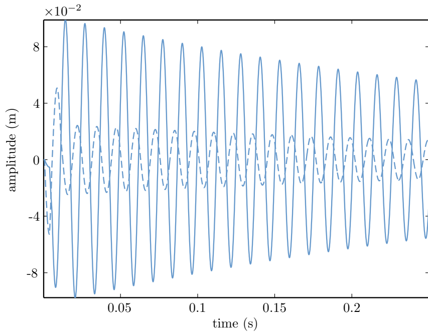
Figure 10: Vibrations of the two modes of the bladed disk for \Omega = 350.2 rad/s ( \Omega < \Omega_{cn} ): u_{m,b}^1 (---) and u_{m,b}^2 (—). A decaying behavior of the bladed disk is observed due to the presence of structural damping in the model.
