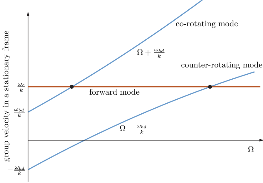
Figure 3: Theoretical modal interaction conditions • as an extension of a Campbell diagram for k -nodal diameter modes. The frequency \omega_c is usually greater than \omega_{bd} of the first flexural mode of the blades. Both lines of equation \Omega \pm \omega_{bd}/k are normally curved as \omega_{bd} is \Omega -dependent: in our study, they are considered as straight lines, meaning that no centrifugal stiffening is accounted for.
