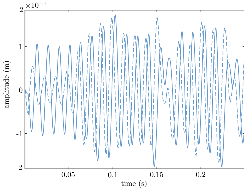
Figure 12: Vibrations of the two modes of the bladed disk for \Omega = 351.4 rad/s ( \Omega \simeq \Omega_{cn} ): u_{m,b}^1 (---) and u_{m,b}^2 (—). A counter-rotating mode propagates in the bladed disk.
