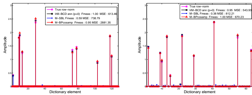
Figure 4: Examples of estimated row-norm using 3 different algorithms. left) M = 128, N = 64, k = 10 and L = 3 . right) M = 64, N = 64, k = 10 and L = 3 . Here, we want to illustrate cases where a “good” sparsity recovery does not necessary lead to low mean-square error.
