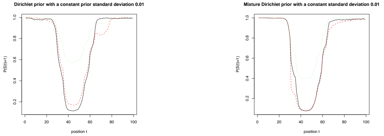
Fig. 2. Posterior probability of each location belonging to segment 1 with r = 3 using Dirichlet prior (left) and mixture Dirichlet prior (right), for the case of fixed standard deviation sd(\lambda_{kk}) = 0.01 and different means: 0.98 (solid line), 0.99 (dashed line) and for 0.995 (dotted line).
