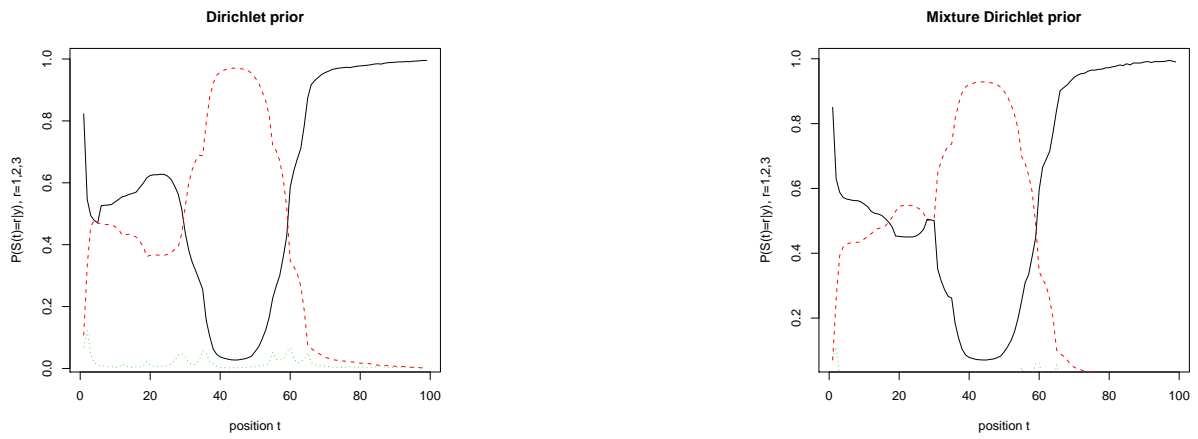
Fig. 3. Posterior probability of each location belonging to each segment type, segment 1 (solid line), segment 2 (dashed line) and segment 3 (dotted line), using Dirichlet prior (left) and mixture Dirichlet prior (right), for the case of fixed mean E(\lambda_{kk}) = 0.99 and fixed standard deviation sd(\lambda_{kk}) = 0.003 .
