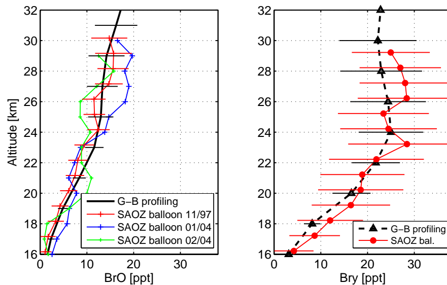
Fig. 9. Retrieved stratospheric BrO profile compared to tropical SAOZ balloon BrO profiles (left plot). Profile of Br γ inferred from ground-based BrO profile compared to the SAOZ balloon Br γ profile at 22° S, November 1997 (right plot).
