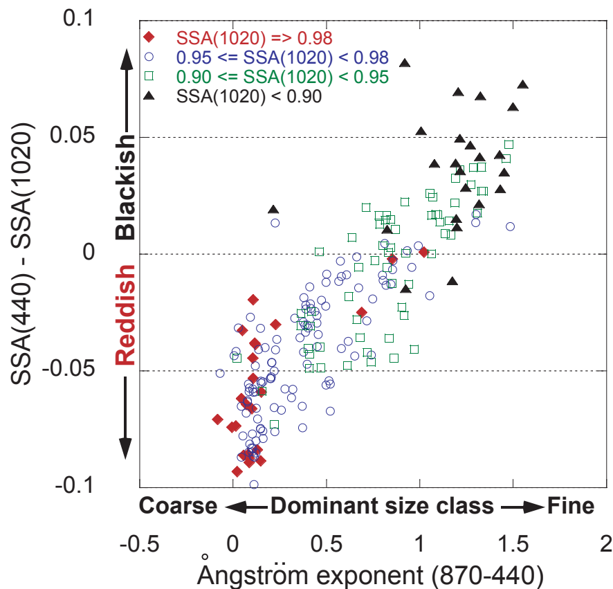
Fig. 2. Difference of SSA(440 \text{ nm}) - SSA(1020 \text{ nm}) versus Ångström exponent. All observations were conducted at the Sede Boker site from October 1995 to May 2006. Different ranges of SSA(1020 \text{ nm}) values are presented by different symbols and indicate events from weak to strong absorption at 1020 nm.
