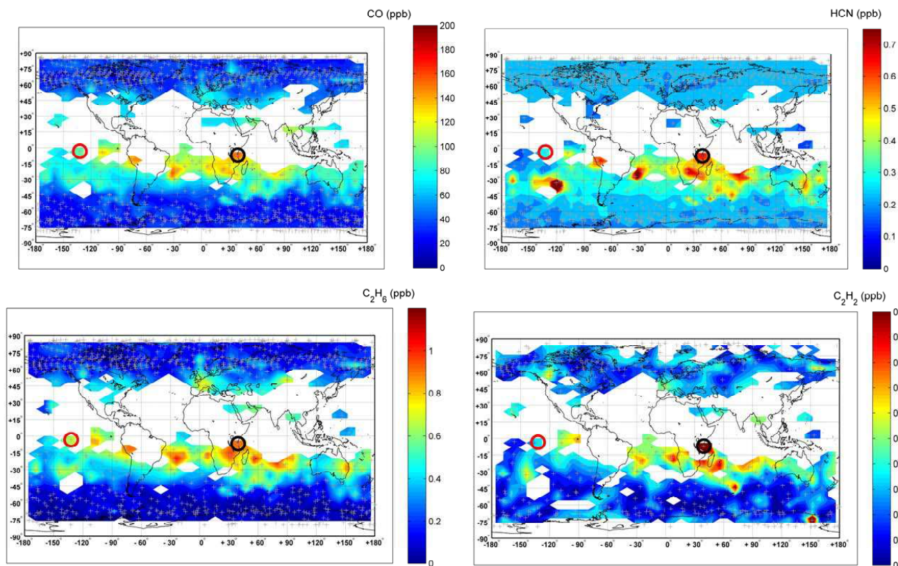
Fig. 1. Zonal distributions of CO, HCN, C 2 H 6 and C 2 H 2 volume mixing ratios at a tangent altitude of 11.5 km, as obtained from the ACE version 2.2 processing. The data are averaged on a 4° latitude × 8° longitude grid using ACE-FTS measurements for the months September to November 2005; the color levels are saturated to highlight the elevated values in the Southern Hemisphere. The crosses identify the ACE measurements locations while the black and red circles shows the location of the fire occultation (ss11607 measured on 8 October 2005 on the East coast of Tanzania), and the background occultation (ss11615 measured on 9 October 2005, at a similar latitude). The ss notation refers to a sunset.
