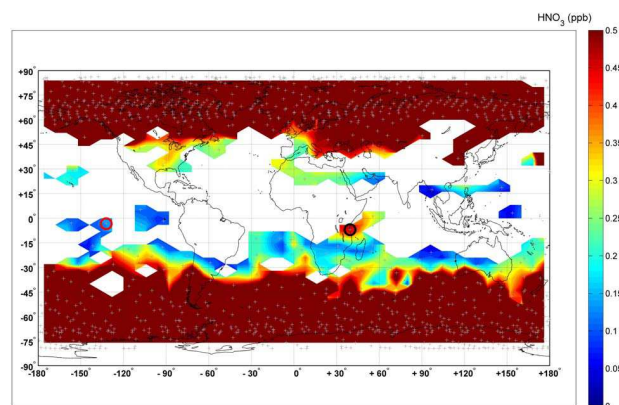
Fig. 2. Same as Fig. 1 for the HNO 3 vmr at 11.5 km.
