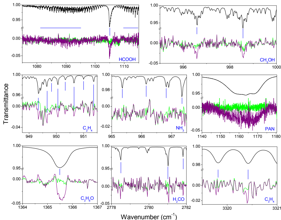
Fig. 5. Spectral fits of the spectrum at a tangent altitude of 11 km (12 km in the case of \text{NH}_3 ) in the regions where weak absorptions are detected, corresponding to contributions of \text{CH}_3\text{OH} , \text{HCOOH} , \text{C}_2\text{H}_4 , \text{NH}_3 , PAN, \text{C}_3\text{H}_6\text{O} , \text{H}_2\text{CO} and \text{C}_3\text{H}_4 . The green and purple lines are the spectral residuals obtained by fitting the observation, respectively, including and excluding the absorption by the target species in the retrieval process. The black lines represent the individual absorption contribution of the molecule and the vertical blue lines indicate the position of the principal spectral features.
