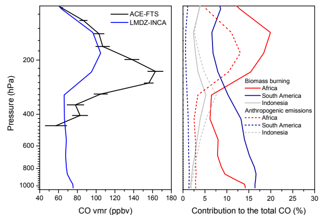
Fig. 4. (left) Comparison between the LMDz-INCA simulated and ACE-FTS measured CO profile for the fire plume (ss11607). The error bars on the ACE-FTS profile show the statistical error associated with the retrieval. (Right) Regional contributions to the total CO, as simulated using LMDz-INCA.
