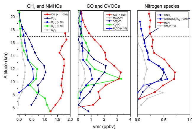
Fig. 6. Volume mixing ratio for several (a) CH_4 and NMHCs, (b) CO and OVOCs and (c) Nitrogen-containing species, found with elevated upper tropospheric concentrations. The dashed lines indicate the tropopause altitude, as inferred from the retrieved temperature profile.
