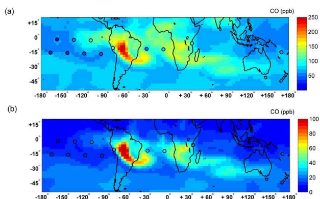
Fig. 3. LMDz-INCA simulations of the CO fields (vmr in ppb) at 250 hPa in the Southern Hemisphere for the 3-day period from 7 October to 9 October 2005. Comparison of (a) the total CO with (b) the biomass burning contribution. Notice the different color scale. The locations of the ACE-FTS occultations during the three days are shown by black circles.
