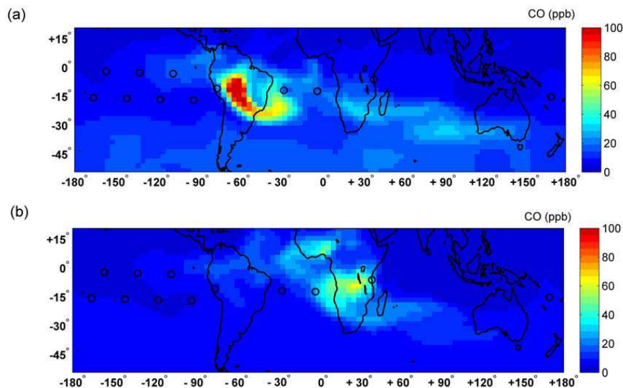
Fig. 4. LMDz-INCA simulations of the CO fields (vmr in ppb) at 250 hPa in the Southern Hemisphere for the 3-day period from 7 October to 9 October 2005. Comparison of the biomass burning contributions to the total CO from (a) South America with (b) Africa. The locations of the ACE-FTS occultations during the three days are shown by black circles.
