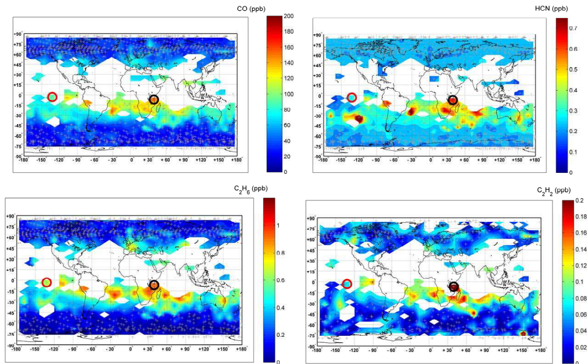
Fig. 1. Zonal distributions of the C_2H_6 , HCN, C_2H_2 and CO volume mixing ratios at a tangent altitude of 11.5 km, as obtained from the ACE version 2.2 processing. The data are averaged on a 4^\circ latitude \times 8^\circ longitude grid and the color levels are saturated to highlight the elevated values in the Southern Hemisphere. The crosses identify the ACE measurements locations while the black and red circles show the location of the fire occultation (ss11607 measured on 8 October 2005 on the East coast of Tanzania), and the background occultation (ss11615 measured on 9 October 2005, at a similar latitude).
