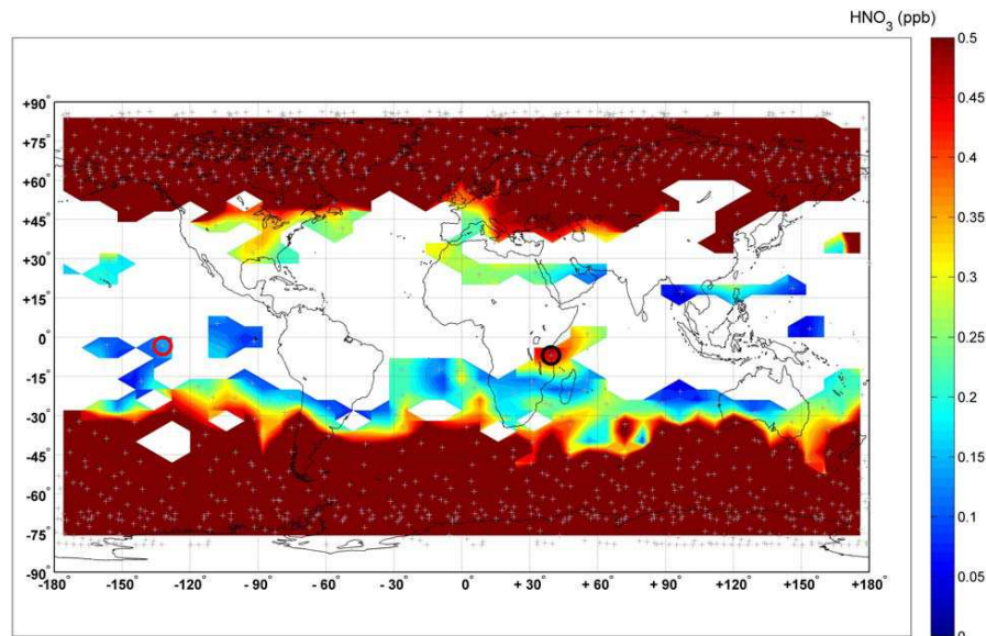
Fig. 2. Same as Fig. 1 for the HNO 3 vmr at 11.5 km.
