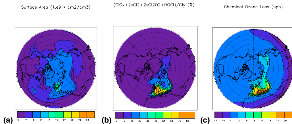
Fig. 3. Maps of PSC, Chlorine activation, and associated ozone loss estimated with numerical simulations. Model-calculated maps of (a) PSC surface area (in \text{cm}^2/\text{cm}^3 ), (b) \text{ClOx}/\text{Cl}_y ratio (active Chlorine species = \text{Cl} , \text{ClO} , \text{Cl}_2 , \text{Cl}_2\text{O}_2 , \text{HOCl} ) and (c) cumulative ozone loss (in ppb over the previous 12 h) at 462 K, on 19 January at 12:00 UT.
