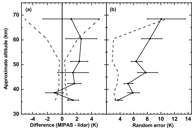
Fig. 12. Plot summarizing the agreement between temperatures of MIPAS and lidar measurements operated by the University of Bonn from Esrang. The format of the plot is the same as Fig. 1.
