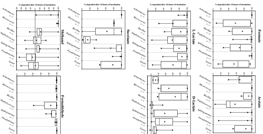
Fig. 3. Percentages of biodegradation for each compound by main genera of bacteria and total yeasts found in cloud water, after 24 h of incubation ( Arthrobacter , Micrococcus , Bacillus , Staphylococcus , Sphingomonas and Pseudomonas and yeasts). Boxes represent medians (—) and 25–75 percentiles; □ means; × minima and maxima. The number of strains considered in each case is indicated. Median is not precised when n < 5 .
