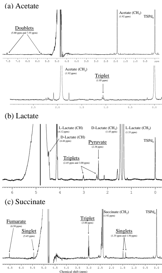
Fig. 5. Examples of ^1\text{H} NMR spectra showing signals appearing during incubation with acetate (a) , lactate (b) and succinate (c) . Spectra presented on (a) were obtained with strains of Bacillus sp. (upper trace) and Curtobacterium flaccumfaciens (lower trace); on (b) Pseudomonas viridiflava and on (c) Curtobacterium flaccumfaciens . The large signal around 5 ppm corresponds to the peak of water.
