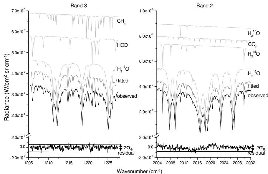
Fig. 1. Spectral micro-windows used for retrieving H 2 16 O, H 2 18 O and HOD profiles. Top and middle: IMG radiance spectra and principal individual contributions of the main absorbers in the IMG band 2 and band 3 spectral ranges. Bottom: Residuals (observed-calculated spectra), plotted with an expanded scale and compared to the \sigma_e value.
