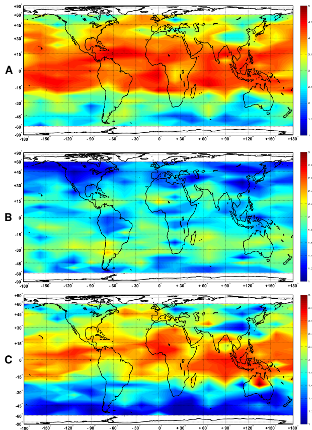
Fig. 5. Global distribution of the DOFS. From top to bottom, H 2 16 O (a), H 2 18 O (b) and HOD (c), averaged on a 10° × 5° longitude-latitude grid, for the 1–10 April 1997 period.
