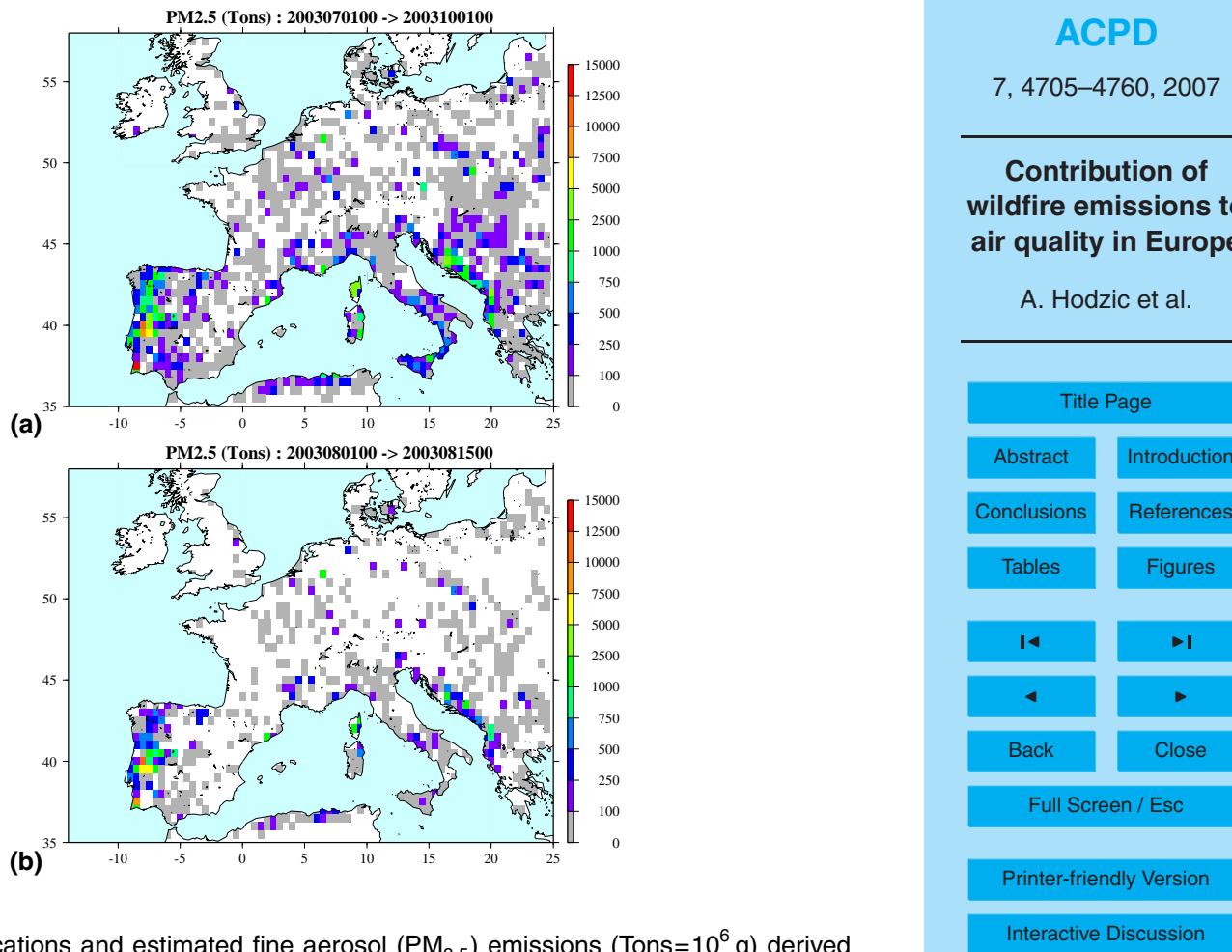
Fig. 2. Wildfire locations and estimated fine aerosol (PM 2.5 ) emissions (Tons=10 6 g) derived from MODIS data over Europe for (a) 1 July to 31 September 2003, and (b) the heat-wave episode, 1 August to 15 August 2003. The map also represents the CHIMERE model domain.
